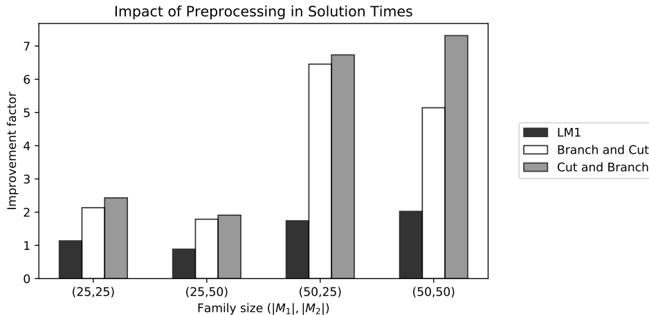
Figure 7: Improvement in solution times for (LM_1) , Branch-and-Cut and Cut-and-Branch.
