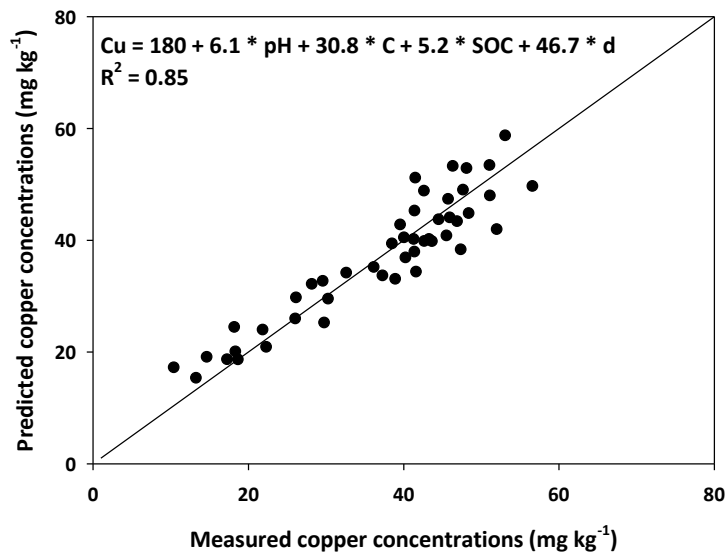
Fig. 8. Measured and predicted copper (Cu) concentrations in topsoil of an organic and an integrated orchard with depth (for details on depth intervals refer to text) using multiple linear regression modelling with pore network (equivalent pore diameter, d , and pore circularity, C ) and basic soil parameters (pH and organic carbon content, SOC). The solid line represents the 1 : 1 line.
