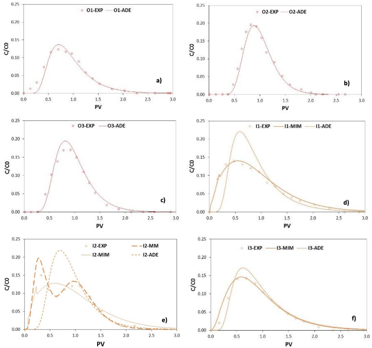
Fig. 4. Experimental data (EXP) and results of the OM-MADE modelling results for the three repetitions of the transport experiments with bromide and the organic (a) O1 (b) O2 (c) O3 and the integrated (d) I1 (e) I2 (f) I3 kiwifruit orchard soil. The following model types were applied: (1) advection-dispersion equation (ADE), (2) mobile-immobile model (MIM), and (3) mobile-mobile model (MM). Results of the best fits for each soil core and the ADE model are shown.
