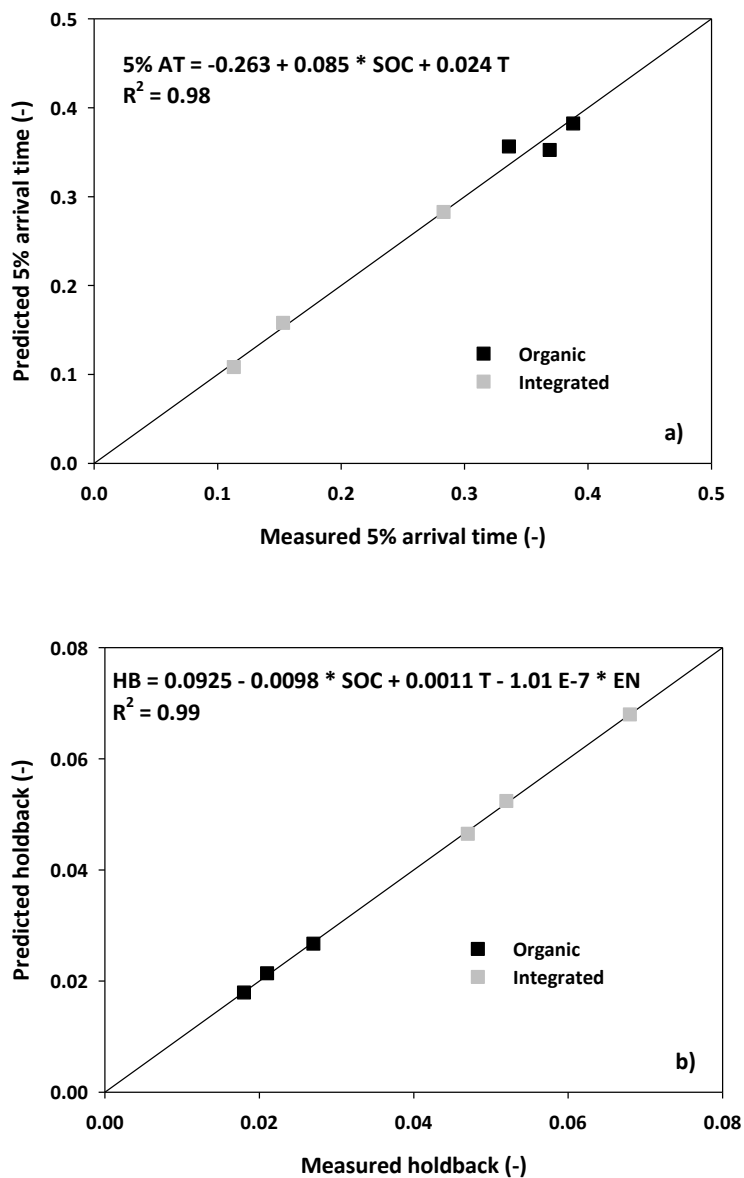
Fig. 6. Relationships between functional and structural soil parameters: (a) measured and predicted 5% arrival time (AT), and (b) measured and predicted holdback factor (HB) considering the pore network parameters connectivity (EN) and tortuosity (T) and carbon (SOC) in a multiple regression analysis. The solid line represents the 1 : 1 line.
