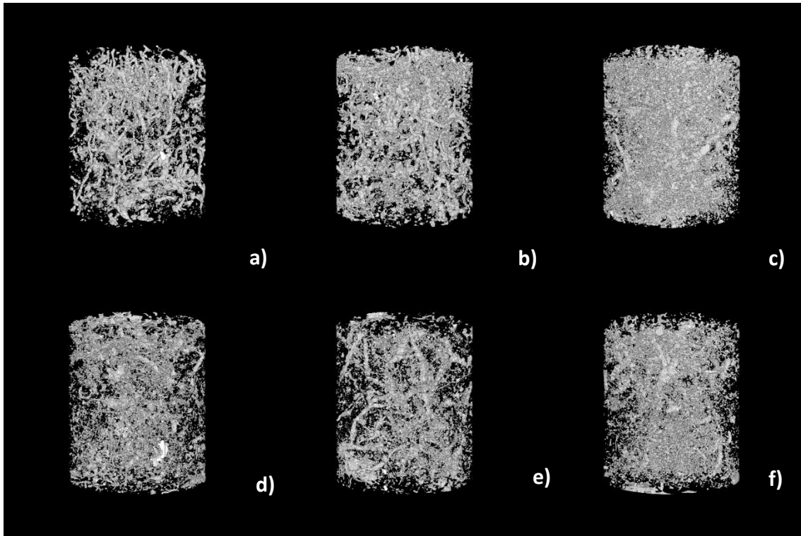
Fig. 2. 3D-macropore network determined via X-ray computed tomography in intact soil cores collected from vine rows of the organic ( a-c ) and the integrated kiwifruit orchard ( d-f ). Pores >92 \mu\text{m} were considered as macropores in this study.
