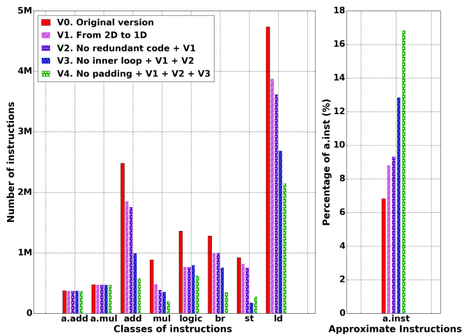
Figure 3: Sobel filter instructions
