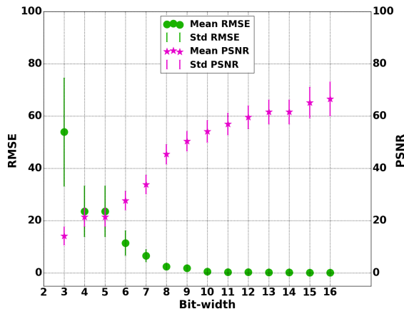
Figure 4: RMSE and PSNR between the reference image and the approximate image
