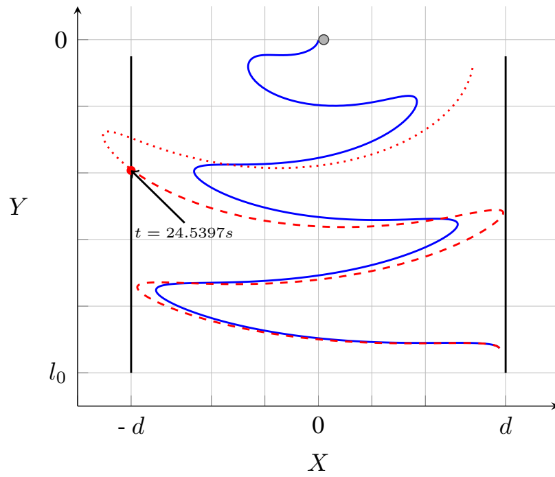
Fig. 14: Trajectories of the system within an enclosed zone for two cases: Case ① (solid line —); Case ② Before impact:(dashed line - - -), After impact: (dotted line ····); Final position without impact ( ● )
