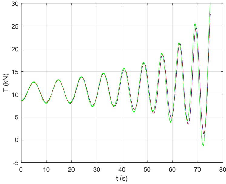
Fig. 8: Tension for different friction and support parameters: \mu = 0 , R = 0 (dashed line - - -) ; \mu = 0.4 , R = 0 (solid line — blue) ; \mu = 0.4 , R = 2 m (solid line — green) Results are obtained from direct numerical integration of Eq. (19)
