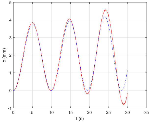
Fig. 3: Time histories of the elongation x ; (solid line \text{---} ), obtained from Eq. (31); (dashed line \text{- - -} ) evaluated from numerical integration of Eq. (19). The effects of friction and the radius of the support are ignored i.e. (\mu, R) = (0, 0)
