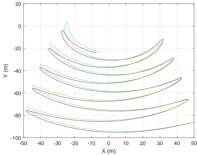
Fig. 7: Mass trajectory for different friction and support parameters: \mu = 0 , R = 0 (dashed line ---) ; \mu = 0.4 , R = 0 (solid line —) ; \mu = 0.4 , R = 2\text{ m} (solid line —) . Results are obtained from direct numerical integration of Eq. (19)
