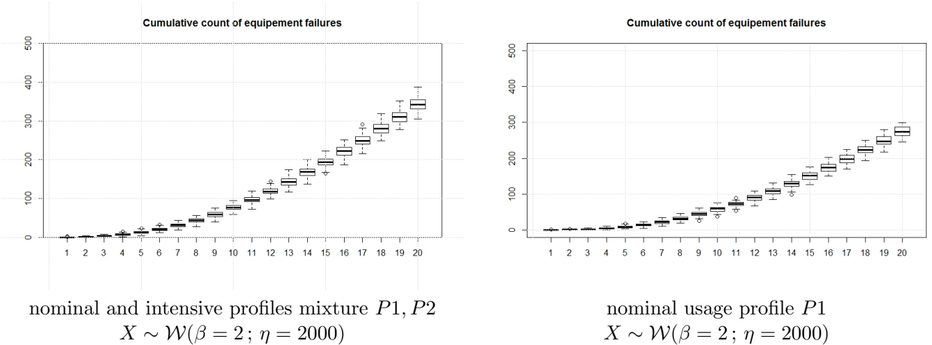
Figure 7: Cumulative count of failures with simple Weibull
