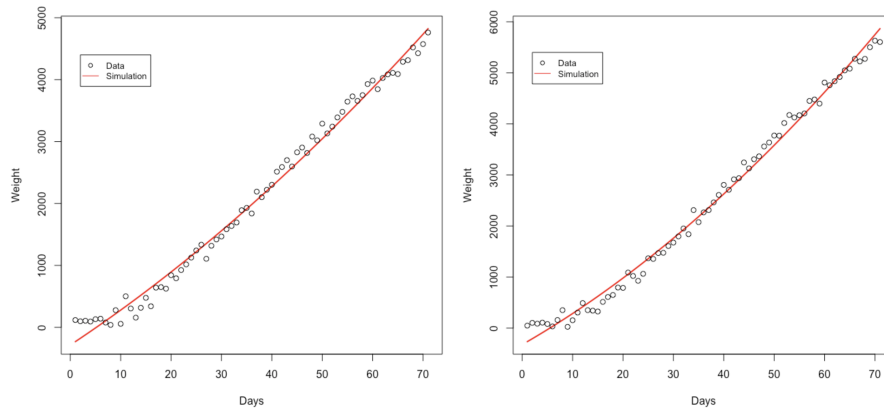
FIGURE 6. Comparison between the initial curve (Data) and the curve simulated via the Gompertz's Model (Simulation) for the Female (left) and the Male Model (right).
