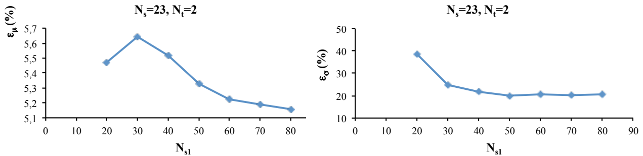
FIG.5- Effect of N_{s1} on \varepsilon_u and \varepsilon_\sigma .
