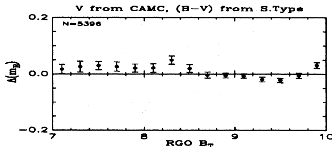
Fig. 9. Differences between RGO and INCA in B_T as a function of B_T and differences in V_T as a function of V_T for stars with photoelectric V and B - V derived from spectral type
