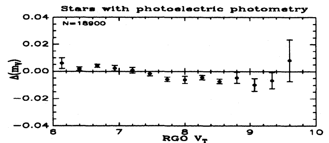
Fig. 8. Differences between RGO and INCA in B_T as a function of B_T and differences in V_T as a function of V_T for stars with photoelectric photometry and V_T < 9.5
