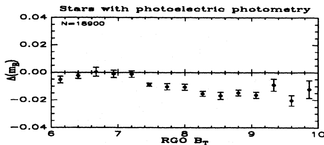
Fig. 8. Differences between RGO and INCA in B_T as a function of B_T and differences in V_T as a function of V_T for stars with photoelectric photometry and V_T < 9.5
