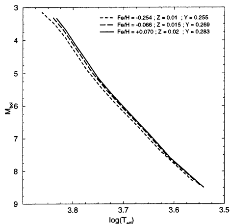
Figure 3. ZAMS computed for different values of Z and Y following Y = 2.8Z + 0.227 .
