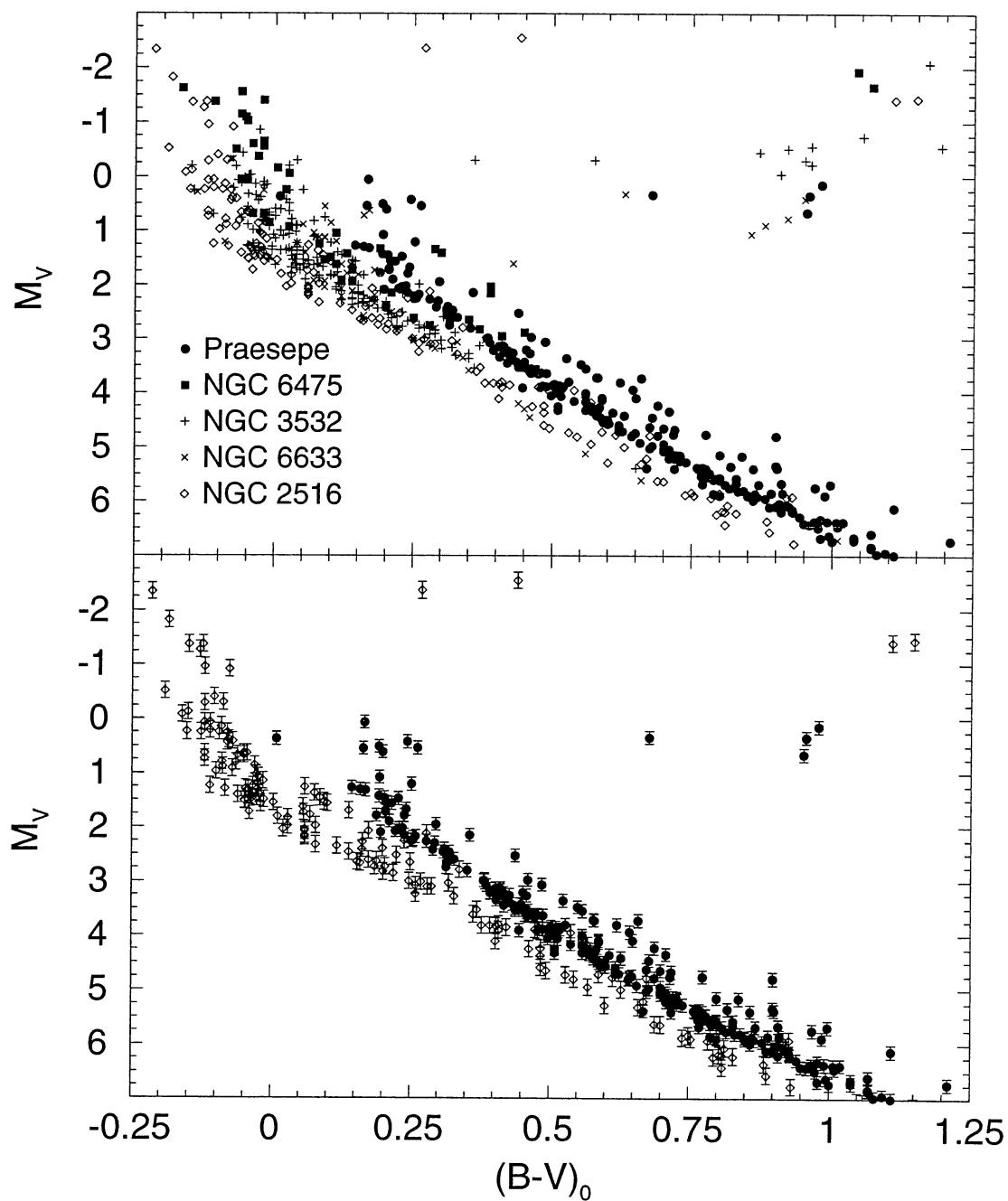
Figure 2. Colour-Magnitude diagram of five open clusters using Hipparcos mean parallaxes.
