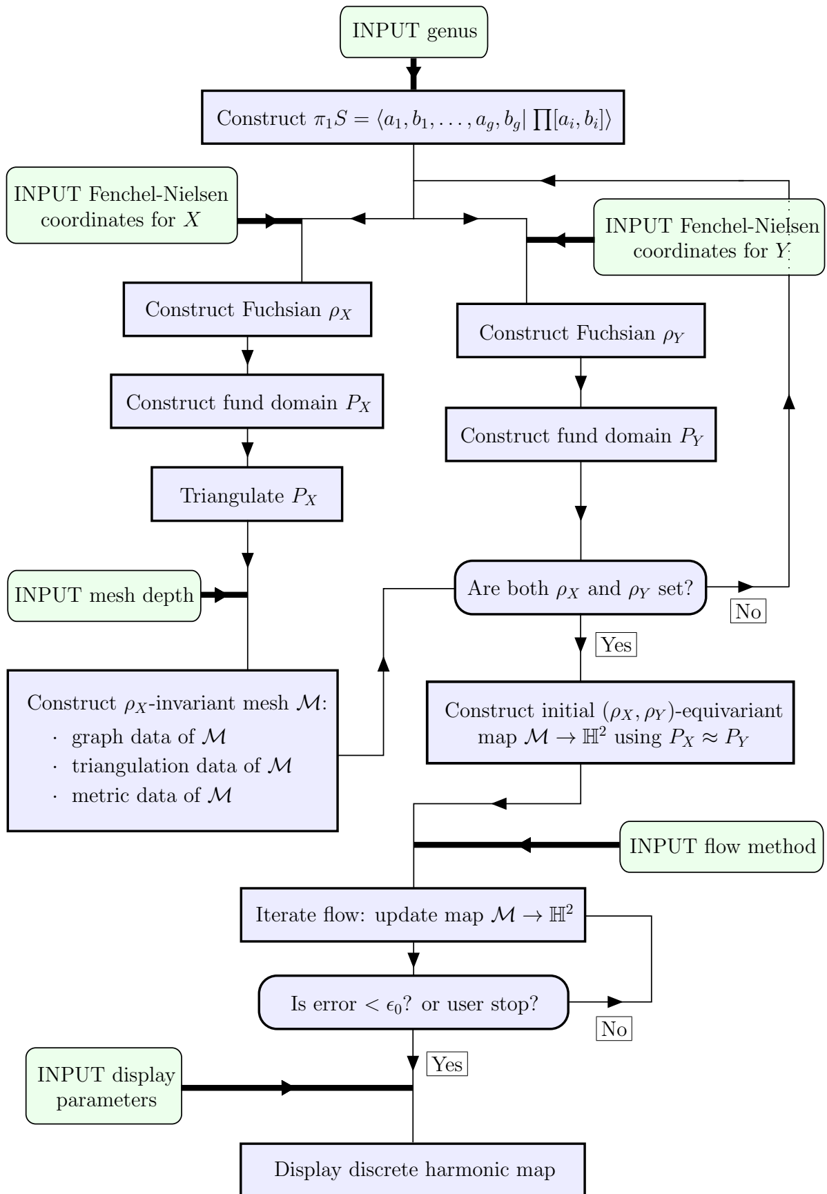
Figure 13: Flowchart representing Harmony's main algorithms.
