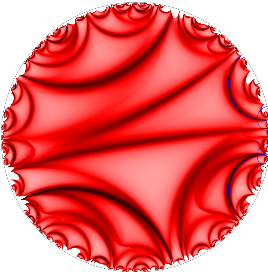
Figure 12: Sample output high energy equivariant harmonic map.
