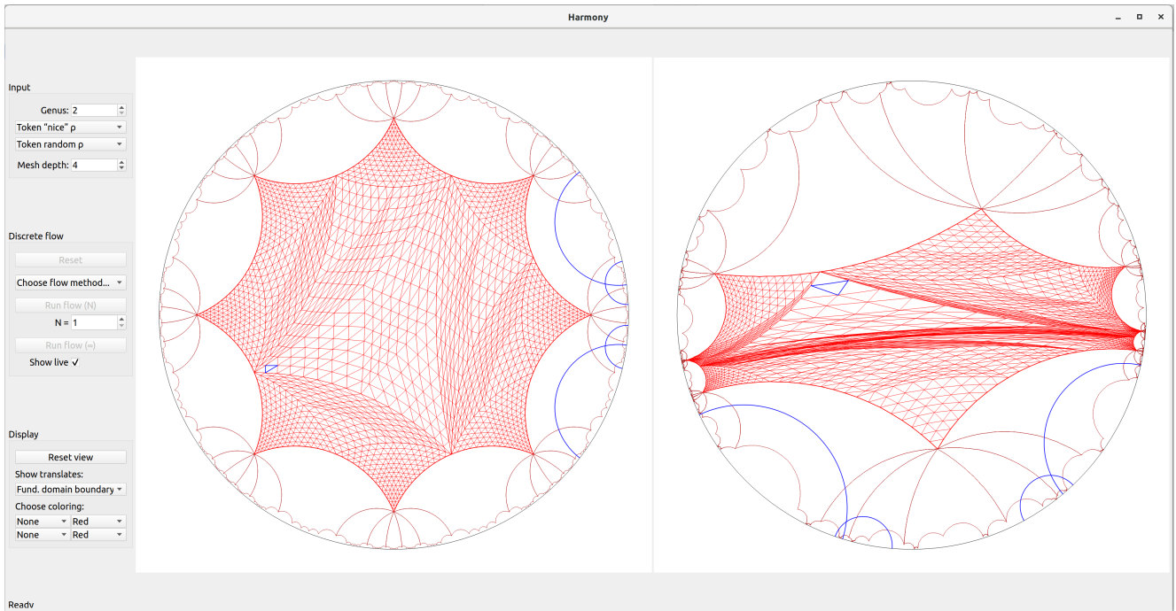
Figure 9: An initial discrete equivariant map f_0 . The highlighted blue triangles are matched.
