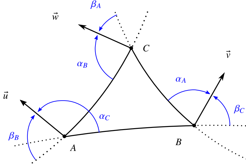
Figure 4: Oriented angles for the tangent vectors to triangle ABC .
