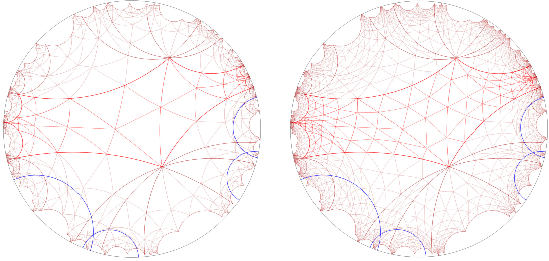
(a) An invariant mesh of \mathbb{H}^2
