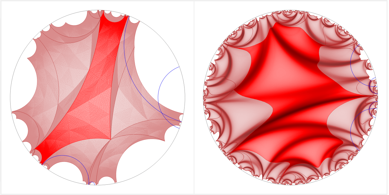
Figure 11: Sample output harmonic map. The brighter central regions are fundamental domains.
