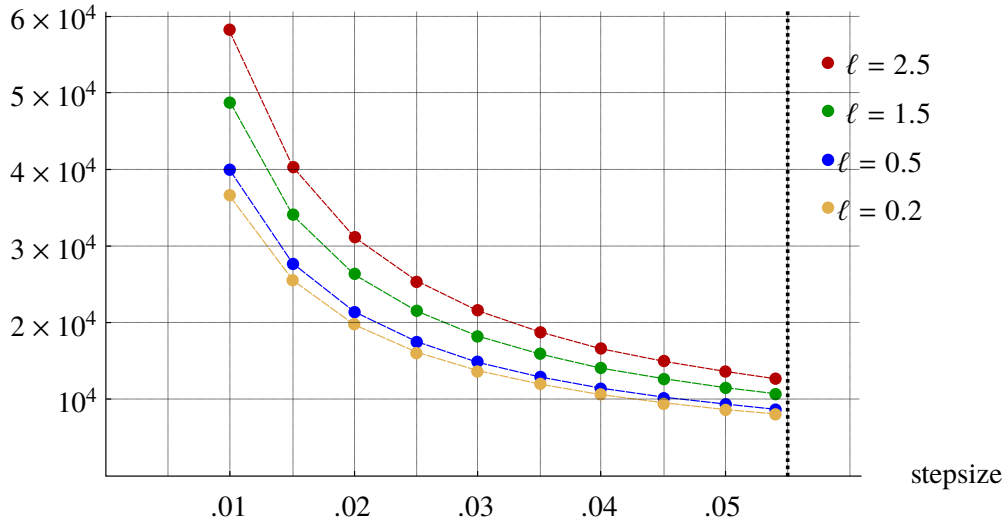
Figure 5: Number of iterations against stepsize in the discrete heat flow with fixed stepsize performed by Harmony.
