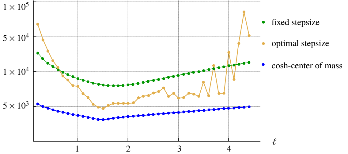
Figure 6: Comparison of the three methods performed by Harmony.
