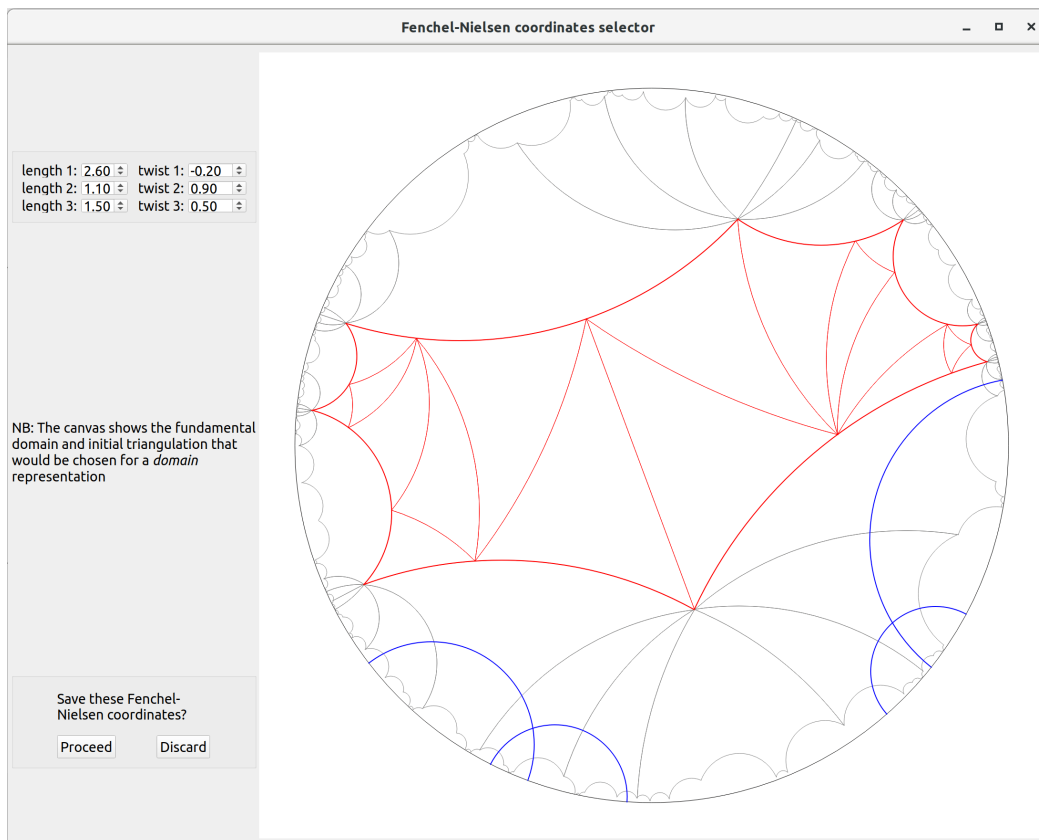
Figure 8: Fenchel-Nielsen coordinates selector.
