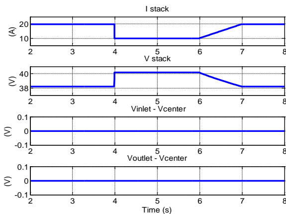
Fig. 9. Principle of monitored cells: healthy stack with current variation.
