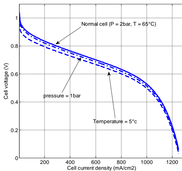
Fig. 5. Polarization curve with different operating conditions.
