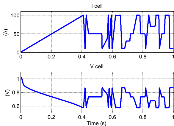
(A) Current and voltage during load cycle.
