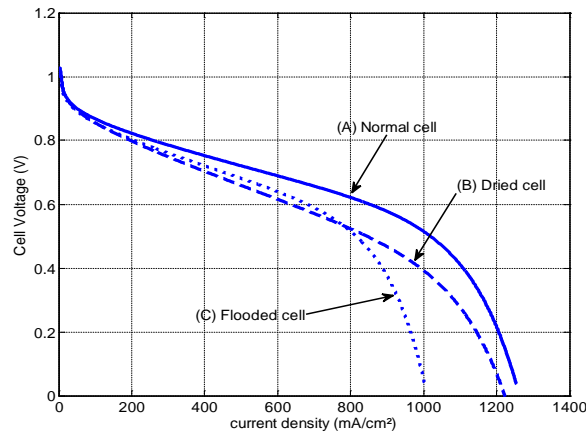
Fig. 2. Different polarization curves of a cell.
