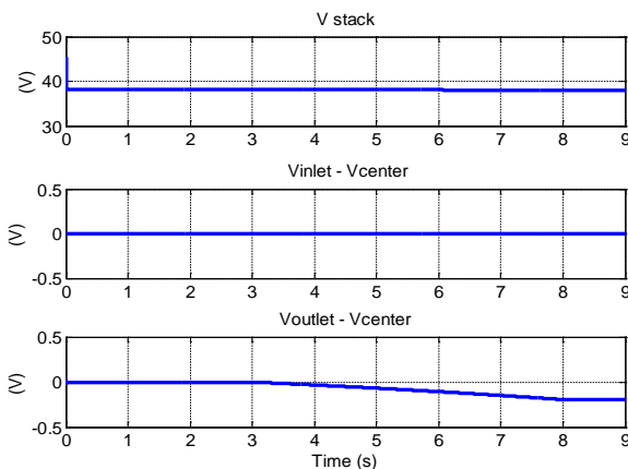
Fig. 7. Principle of monitored cells: flooding case.
