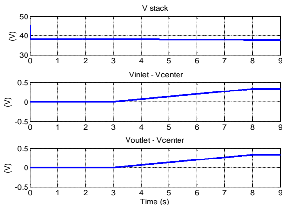
Fig. 8. Principle of monitored cells: drying case.
