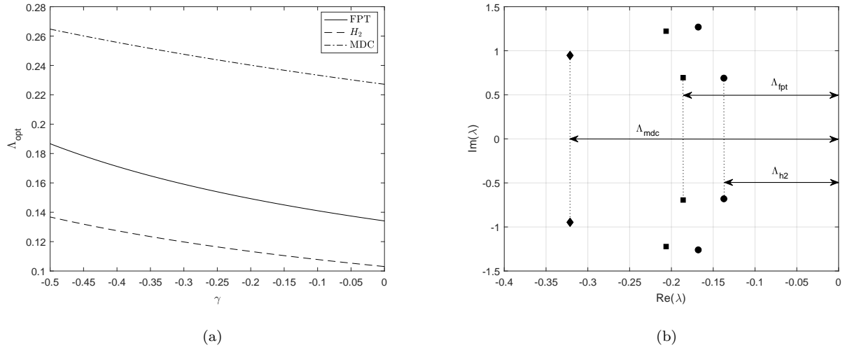
Figure 8: Root locus of characteristic equations relevant to each calibration technique: (a) Optimal decay performance index \Lambda_{opt} as a function of inductance ratio \gamma (solid line: FPT, dashed: H_2 , dash-dotted: MDC); (b) Root location with \gamma = -0.5 (square marker: FPT, circle: H_2 , diamond: MDC).
