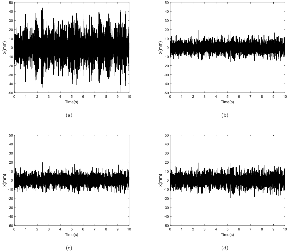
Figure 7: Temporal responses of primary system under random force excitation with \gamma = -0.5 and S_f = 10N^2 \cdot Hz^{-1} : (a) short circuit; (b) FPT; (c) H_2 ; (d) MDC.
