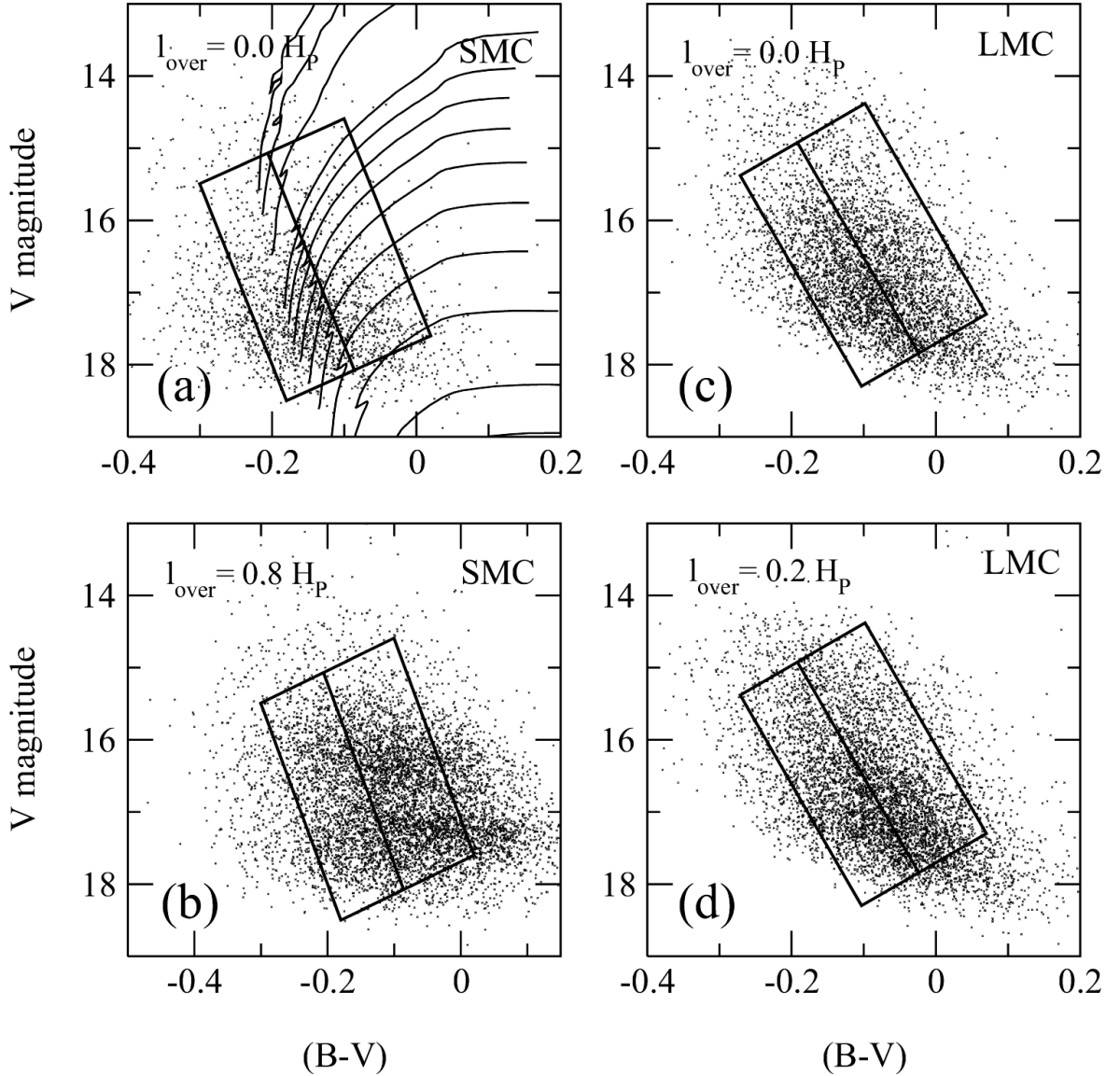
Fig. 3. Synthetic CM-Diagrams for SMC and LMC chemical compositions, panels a ) and b ) are for the SMC with two overshooting amounts: \alpha_{\text{over}} = 0.0 and \alpha_{\text{over}} = 0.8 , panels c ) and d ) are for the LMC with: \alpha_{\text{over}} = 0.0 and \alpha_{\text{over}} = 0.2 respectively. For panel a ) only 30% of the synthetic objects have been displayed for clarity purpose and corresponding evolutionary tracks have been plotted. For other panels: b )– d ) the number of displayed objects has not been reduced. In all cases the total number of stars in the boxes -used for calculations- is close to the observational one: a ) N_1 + N_2 = 4403 ( N_2/N_1 = 0.65 ), b ) N_1 + N_2 = 5011 ( N_2/N_1 = 1.59 ), c ) N_1 + N_2 = 3582 ( N_2/N_1 = 0.94 ), d ) N_1 + N_2 = 4717 ( N_2/N_1 = 1.13 ). We recall that empirically we got for the SMC N_1 + N_2 = 4653 ( N_2/N_1 = 1.08 ) and for the LMC N_1 + N_2 = 4113 ( N_2/N_1 = 1.01 ). The ratios N_2/N_1 obtained theoretically are rather independent from the value of N_1 + N_2 in the synthetic CM-Diagram, for instance in the case of the panel b ) we got N_2/N_1 = 1.60 with N_1 + N_2 = 6399 . The cloud of dots in panel b ) ( l_{\text{over}} = 0.8 H_p , SMC) calls a comment: it appears to be bimodal, i.e. showing over-populated regions around V \sim 17.5 mag and V \sim 16.3 mag. Indeed for high overshooting values the main sequence of masses as small as \sim 3 M_{\odot} can reach V \sim 17.5 generating with their large evolutionary time scale an over-populated region. Moreover the binary shifts a part of this population to a \sim 0.8 mag brighter region, with a binarity rate \beta = 0.0 , this “bimodal effect” disappears.
