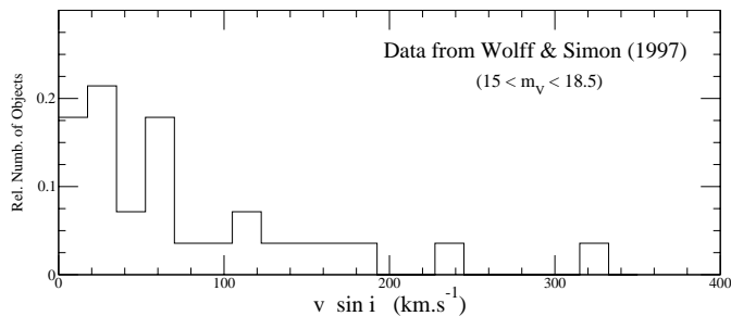
Fig. 6. Relative number of stars ( N_{\text{stars}}/N_{\text{tot}} versus V \times \sin i for Wolff & Simon (1997) objects with magnitudes in our studied range.
