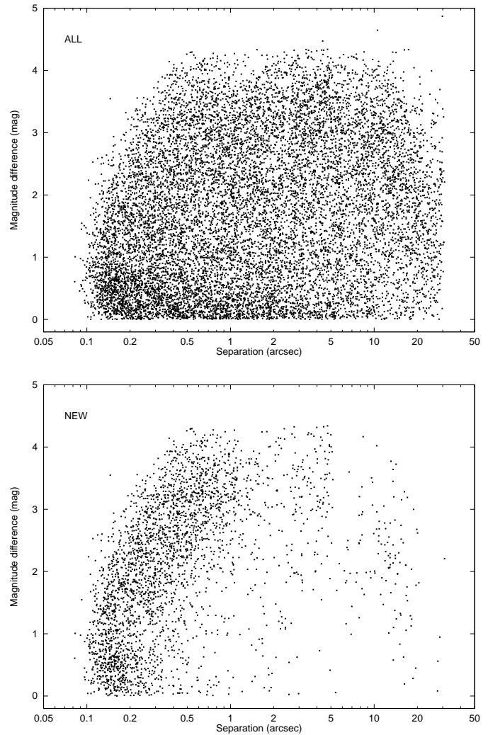
Fig. 1. Distribution of separation and magnitude difference for all 12 393 component pairs in Part C of the Annex (top), and for the subset of 2996 pairs discovered with Hipparcos (bottom)
