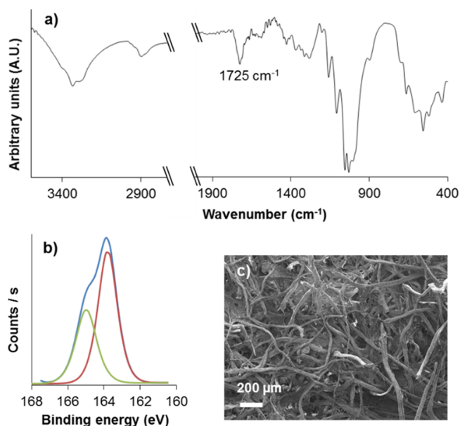
Figure 1. (a) FTIR spectrum, (b) high-resolution S 2p XPS spectrum, and (c) SEM image of Cell-DiS.
