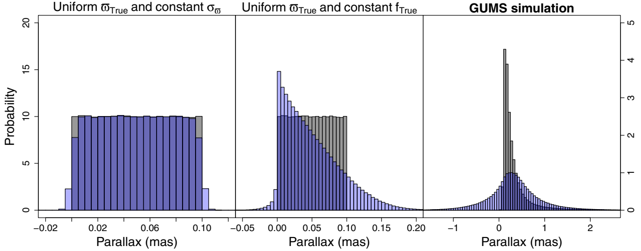
Fig. 10. Histograms of true (grey) and observed (blue) parallaxes for three simulations: uniform distribution of parallaxes and constant \sigma_w = 0.3 mas ( left ); uniform distribution of parallaxes and constant f = 0.5 ( centre ); and the GUMS simulation described in Appendix A ( right ).
