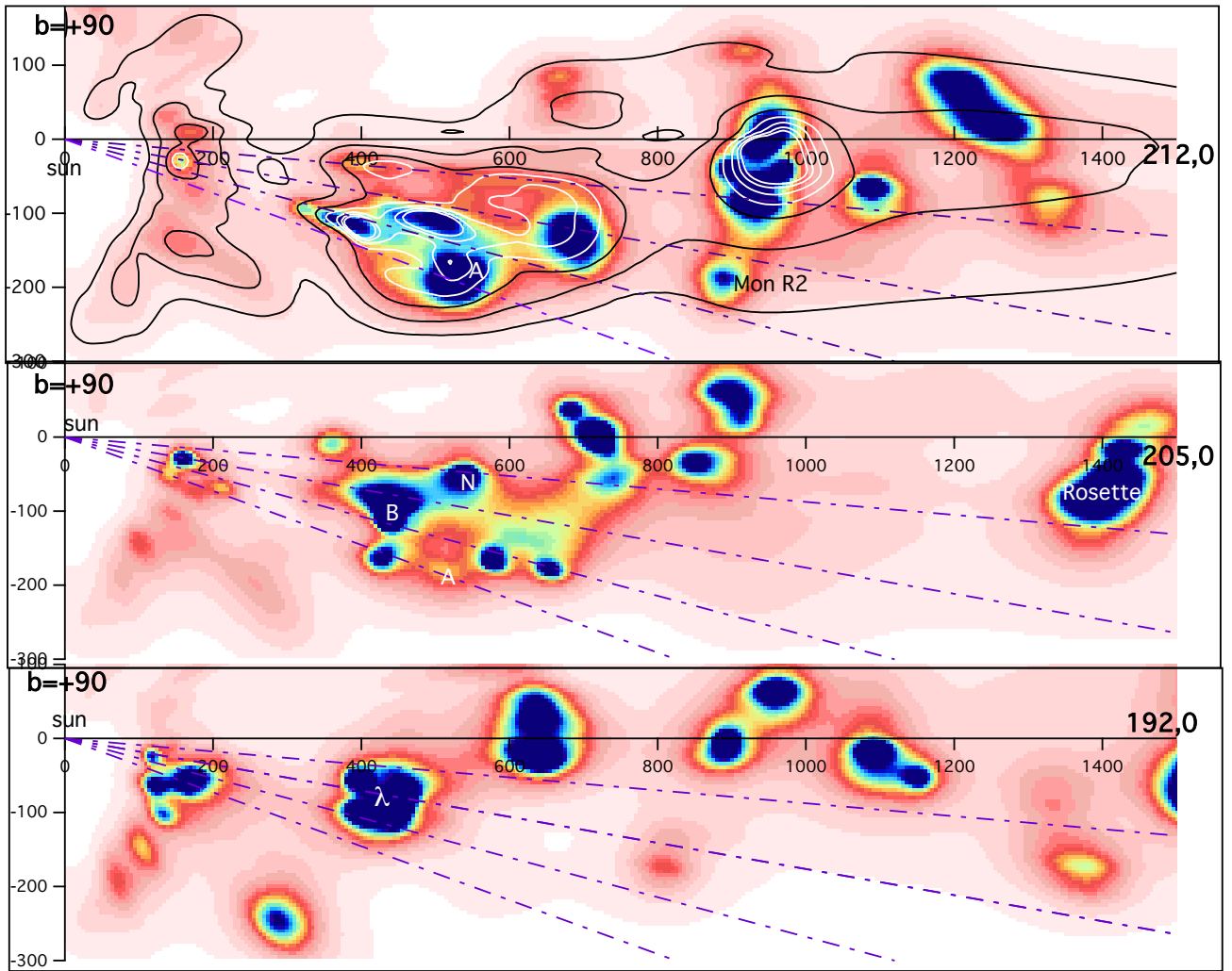
Fig. 10. Differential color excess in a vertical plane containing the Sun and along the Galactic longitudes l = 212^\circ , 205^\circ , and 192^\circ from top to bottom. The maps show the distribution of the main Orion clouds. Superimposed as black or white lines on the top graph are isocontours of the differential color excess from the previous inversion of Capitanio et al. (2017). The new 3D distribution reveals more clouds at large distance (e.g., the clouds beyond 800 pc) and resolves more structures in the main Orion region between 400 and 700 pc. We indicate the structures A, B, N as well as \lambda Ori, Mon R2, and Rosette at the locations predicted by Lombardi et al. (2011) and Schlafly et al. (2015).
