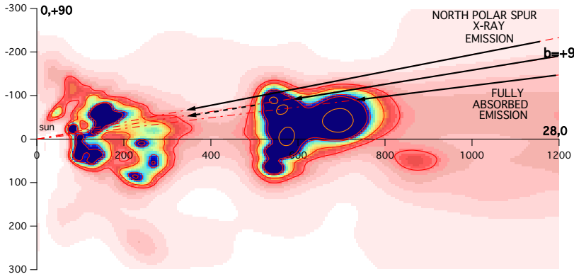
Fig. 9. Differential color excess in a vertical plane containing the Sun and along the Galactic longitude l = 28^\circ . The north Galactic pole is at the top. The map shows the distribution of the North Polar Spur (NPS) X-ray emission and fully absorbed emission. The b = +9^\circ dashed line corresponds to the latitude above which X-rays from the NPS start being detected. The very thick cloud absorbing predominantly the NPS at b \leq +9^\circ is located between 500 and 800 pc.
