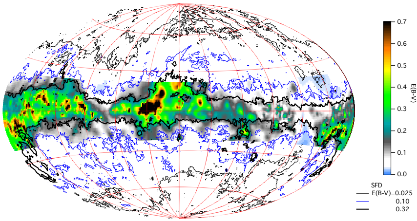
Fig. 5. Same as Fig. 4, for sightlines 800 pc long. Grid points are left blank at high Galactic latitudes ( \text{abs}(b) \gtrsim 25^\circ ); for such sightlines 800 pc distant sightline extremities are out of our 4000 \times 4000 \times 600 \text{ pc}^3 computational volume. In the second quadrant ( 90 \leq l \leq 180^\circ ) there is good agreement between SFD98 isocontours for E(B-V) = 0.32 mag and locations corresponding to about the same value of our integrated color excess. This shows that most of the structures in these areas are within 800 pc. On the contrary, for a large fraction of the third and fourth quadrants ( 180 \leq l \leq 270^\circ and 270 \leq l \leq 360^\circ , respectively) most of the dust seen in emission is beyond 800 pc.
