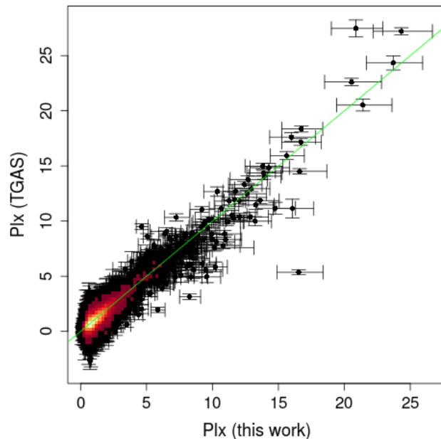
Fig. 1. Comparison of photometric distances obtained in this work with the Gaia /TGAS parallax distances for 13451 APOGEE stars. The color scale represents the square root of the density of stars, with yellow (resp. black) for the highest (resp. lowest) density.
