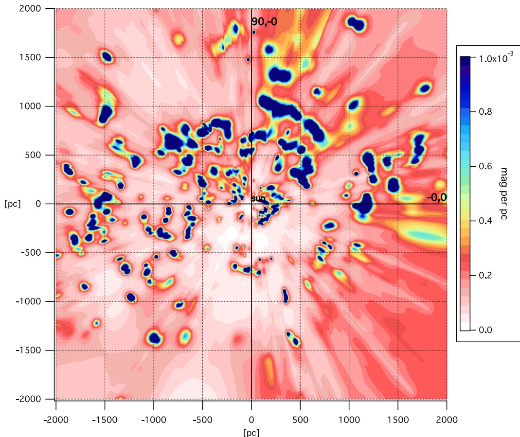
Fig. 7. Differential color excess in the Galactic plane computed as a planar cut along the Galactic equator through the 3D distribution. The Sun is at the center of the image (coordinates 0, 0). The Galactic center direction is to the right. The units are \text{mag pc}^{-1} . The map can be directly compared with the previous similar map from Capitanio et al. (2017).
