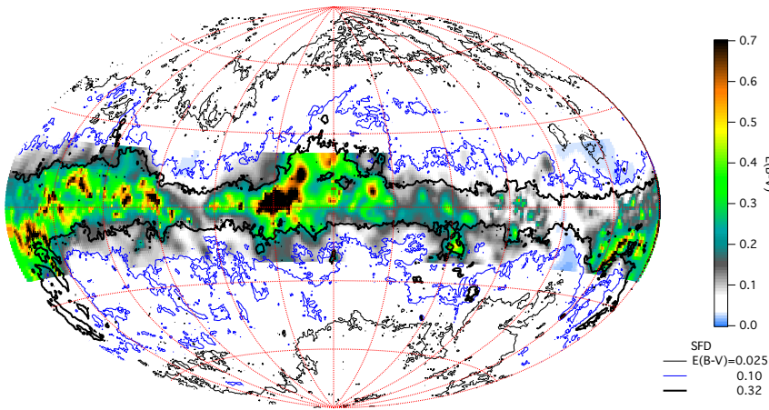
Fig. 5. Same as Fig. 4, for sightlines 800 pc long. Grid points are left blank at high Galactic latitudes ( \text{abs}(b) \geq 25^\circ ); for such sightlines 800 pc distant sightline extremities are out of our 4000 \times 4000 \times 600 \text{ pc}^3 computational volume. In the second quadrant ( 90 \leq l \leq 180^\circ ) there is good agreement between SFD98 isocontours for E(B-V) = 0.32 mag and locations corresponding to about the same value of our integrated color excess. This shows that most of the structures in these areas are within 800 pc. On the contrary, for a large fraction of the third and fourth quadrants ( 180 \leq l \leq 270^\circ and 270 \leq l \leq 360^\circ , respectively) most of the dust seen in emission is beyond 800 pc.
