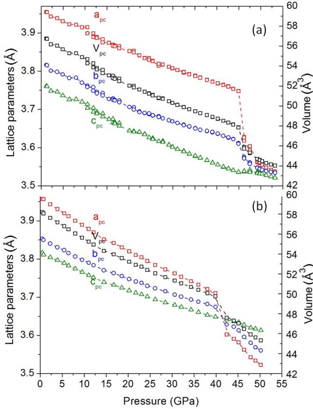
FIG. 1. Pseudocubic lattice parameters and volume as a function of pressure for (a) \text{TbFeO}_3 and (b) \text{SmFeO}_3 . The dashed lines are guides for the eyes.
