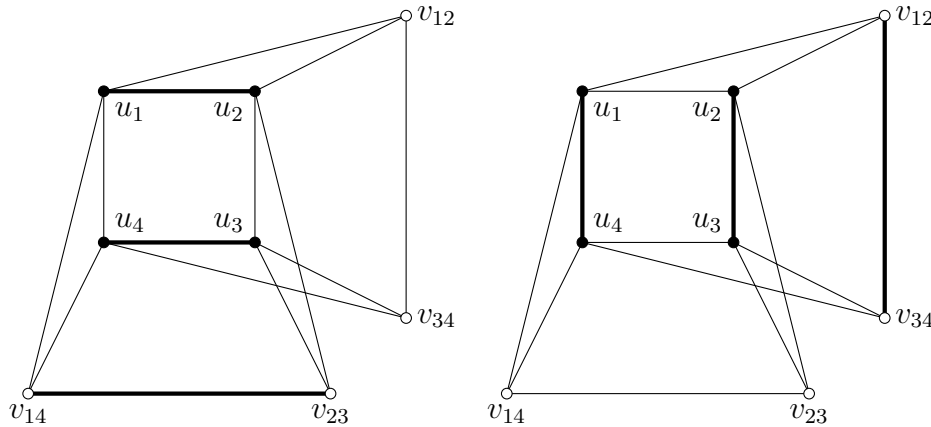
Figure 2: The variable gadget, and the two possible sets of edges in M (the thick edges).
