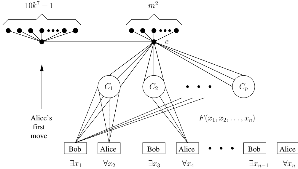
Figure 4: The general construction of G' from an Alternating QSAT instance using the clause sets C_i and Bob and Alice gadgets. The Bob and the Alice gadgets are connected to the clause sets according to the formula F , but note that the details of this construction are more complicated: only a certain subset of the vertices of the Bob or Alice gadget corresponding to variable x_j is connected to the clause sets in which x_j appears, and another subset of vertices is connected to the clause sets in which \bar{x}_j appears, with the rest of the vertices in the gadget not being connected to any clause set. See the details of the construction on page 14. This construction is made to guarantee that, in the first phase of the game, the players are forced to play in the Alice and Bob gadgets from left to right (three moves in a Bob gadget by Bob, Alice, and then Bob again, and one move in an Alice gadget by Alice) and not to play in a clause set, unless they would like to lose immediately. See Figures 5 and 6 for the details of the Bob and Alice gadgets.
