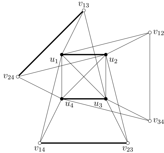
Figure 3: The clause gadget, with one of the three possible sets of edges in M (the thick edges).
