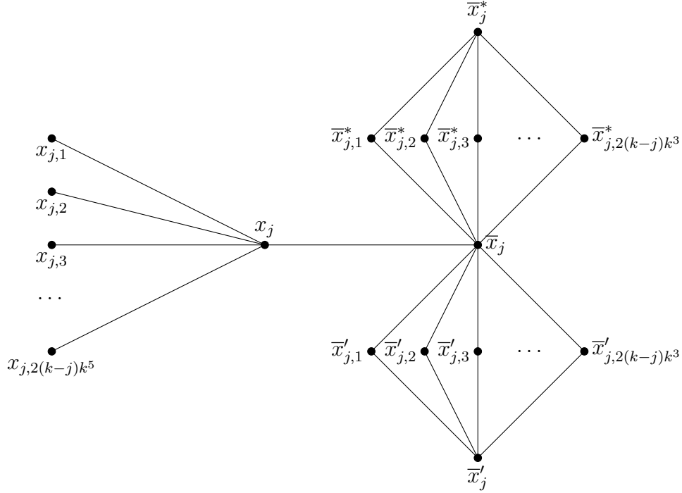
Figure 6: An Alice gadget.
