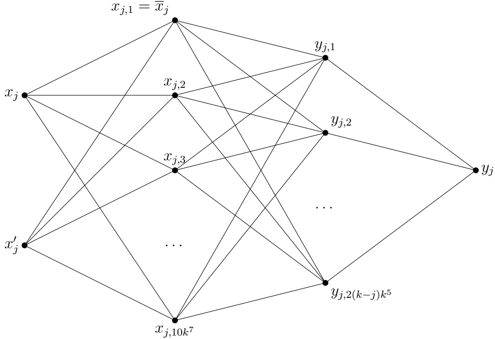
Figure 5: A Bob gadget.
