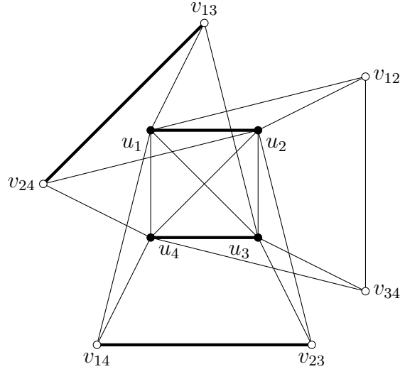
Figure 3: The clause gadget, with one of the three possible sets of edges in M (the thick edges).
