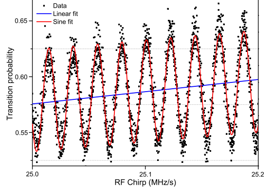
FIG. 5. Effect of slope on fringe offset. The blue line is the estimated fringe offset P_m = P_{m0} + 2\pi A\alpha .
