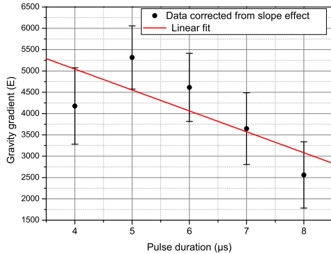
FIG. 8. Variation of the gravity gradient value due to two-photon light shift (TPLS) versus \pi/2 -pulse duration keeping Rabi frequency \Omega constant. The Raman \pi -pulses are kept constant to preserve the interferometer's contrast. All data points are corrected from the effect of the slope on fringe offset. The slope given by the fit is -490 \text{ E}/\mu\text{s} .
