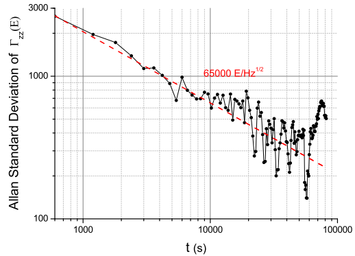
FIG. 2. Allan standard deviation of the gravity gradient measurements. The dash line illustrates the t^{-1/2} scaling.
