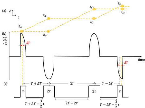
FIG. 6. (a): Space-time diagram of atom classical trajectory for the 4 pulses AI in absence of gravity. We consider that the path separation occurs at the exact value of the position response during the pulse ( t_{sep} = \int_0^\tau f_p(t) dt ). This separation time corresponds to the moment where the laser phase is imprinted on the atom wave function assuming that the laser phase has a linear time dependence during laser pulse. (b) Position response function f_p(t) of the four-pulse AI considering finite Raman pulses [44]. (c) Timing diagram of the four pulse AI defining time with respect to the center of the Raman light-pulse.
