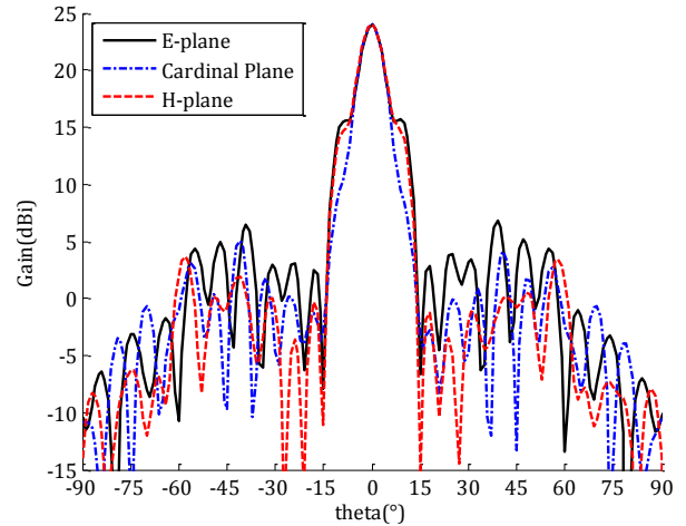
Fig. 4. Simulated co-polarized gain components of the MOTA at 19 GHz.
