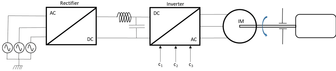
Fig. 1. Electromechanical chain
