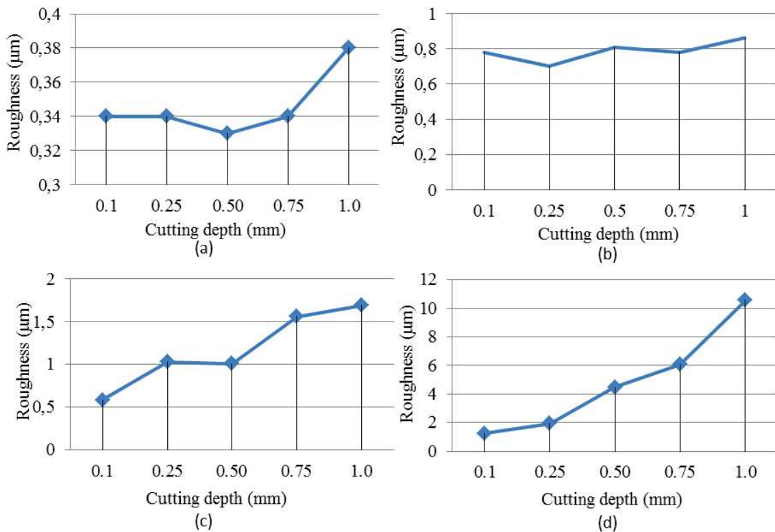
Fig.8. Roughness (experimental): (a) 0° fiber orientation (b) 45° fiber orientation (c) 90° fiber orientation and (d) at 135° fiber orientation.
