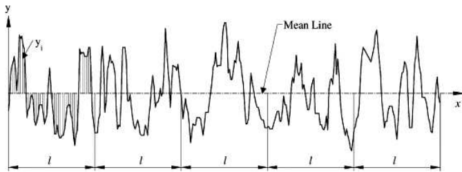
Fig.7. Arithmetic average height, R_a [Gadelmawla et al., 2002].
