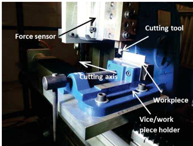
Fig.3. Experimental setup
