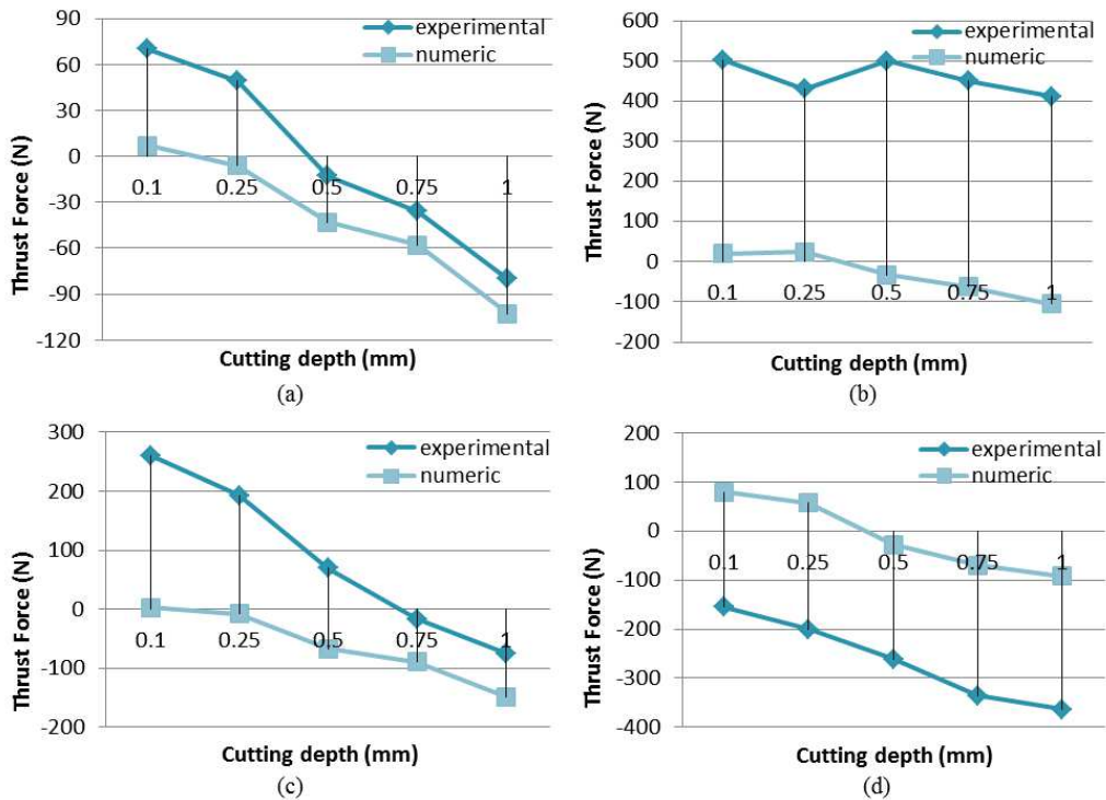
Fig.5. Comparison of numerical and experimental thrust forces: (a) 0^\circ fiber orientation (b) 45^\circ fiber orientation (c) 90^\circ fiber orientation and (d) at 135^\circ fiber orientation.
