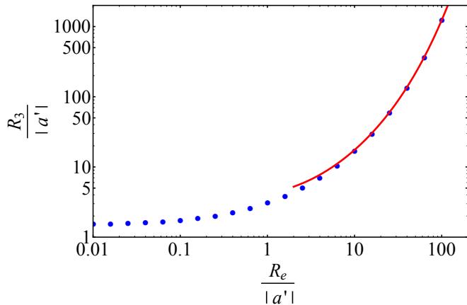
FIG. S4. Blue dots: numerical calculations of R_3/|a'| for different R_e/|a'| ratios and \eta = 7/6 . Red curve: fit for R_e/|a'| \gg 1 using a function A\sqrt{X}\exp\left(\frac{\sqrt{3}}{16\pi^2|\kappa(7/6)|}\sqrt{X}\right) , with A an adjustable parameter. A \simeq 0.8 after optimization.
