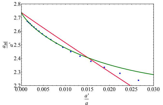
FIG. S5. Blue dots: Points from [7] showing the ratio of the atom-dimer scattering length a_{\text{ad}} over a' , for \eta = 7/6 . Red solid curve: fit to the blue dots using the function a_{\text{ad,Born}}/a'(1 + AX(\ln X + B)) where A is a fixed parameter corresponding to the analytical result obtained through BCS theory ( A \propto \kappa^{\text{MF}} ) and B is an adjustable parameter. Green solid curve: theoretical curve obtained through three-body calculations, its equation is the same as the one used for the red curve but now with A \propto \kappa and B obtained through C_{\text{ad}} and R_3 . We see that the curve corresponding to BCS theory (red) does not match at all the results reported in [7], contrary to the other one (green).
