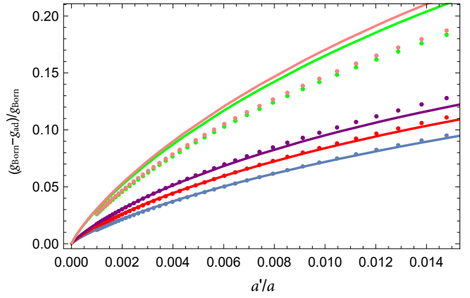
FIG. 3. Atom-dimer s-wave coupling constant relatively to Born's approximation prediction g_{\text{Born}} = 2g' . Dots: numerical resolution of the three-body problem from [40]. From bottom to top: \eta = 7/40 (blue), 23/40 (red), 7/6 (purple), 87/6 (orange), 133/6 (green). Solid line: Asymptotic result Eq. (21) where R_3 and C_{\text{ad}} are computed numerically and are given in [31]. Here R_3 and C_{\text{ad}} are computed taking R_e = 0 and the slight discrepancy observable at large \eta is probably due to the finite range R_e \lesssim a' used in [40] to regularize the three-body problem.
