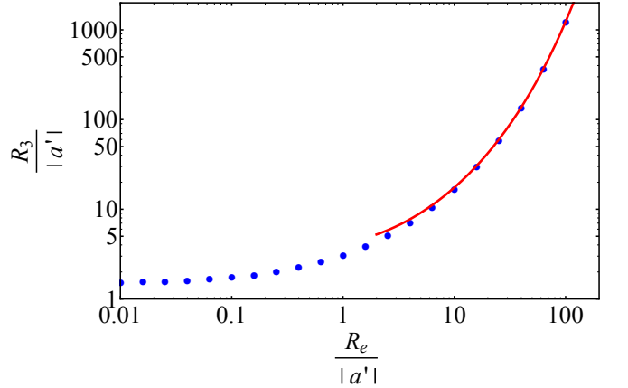
FIG. S4. Blue dots: numerical calculations of R_3/|a'| for different R_e/|a'| ratios and \eta = 7/6 . Red curve: fit for R_e/|a'| \gg 1 using a function A\sqrt{X} \exp\left(\frac{\sqrt{3}}{16\pi^2 |\kappa(7/6)|} \sqrt{X}\right) , with A an adjustable parameter. A \simeq 0.8 after optimization.
