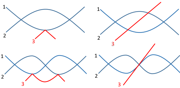
FIG. 2. Singular diagrams at second order of Born's approximation. The red line corresponds to the impurity.
