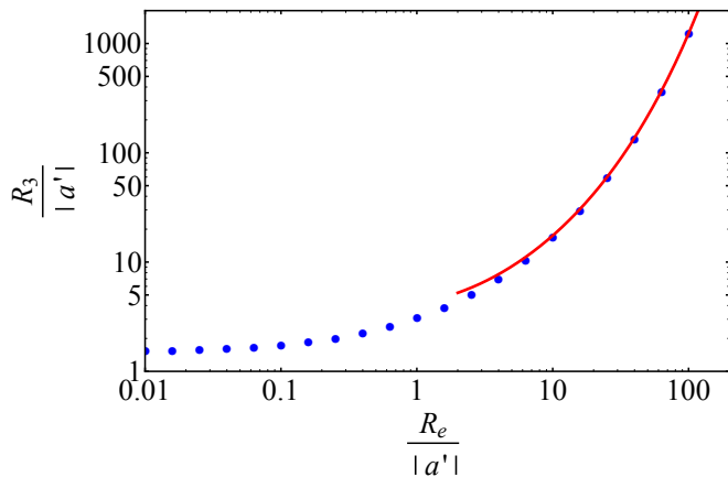
FIG. S4. Blue dots: numerical calculations of R_3/|a'| for different R_e/|a'| ratios and \eta = 7/6 . Red curve: fit for R_e/|a'| \gg 1 using a function A\sqrt{X} \exp\left(\frac{\sqrt{3}}{16\pi^2|\kappa(7/6)|}\sqrt{X}\right) , with A an adjustable parameter. A \simeq 0.8 after optimization.
