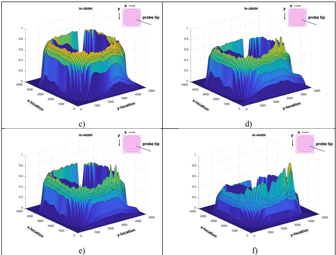
Fig 13. Experimental 2D-mapping of the OBIC current at different voltages (a) 0V, b) 2000V, c) 3500V, d) 3800V, e) 4000V and f) 4400V) for the 400 \mu\text{m} MESA JTE + 8 rings protected diode. The inset gives the x-y direction and the position of the tip.
