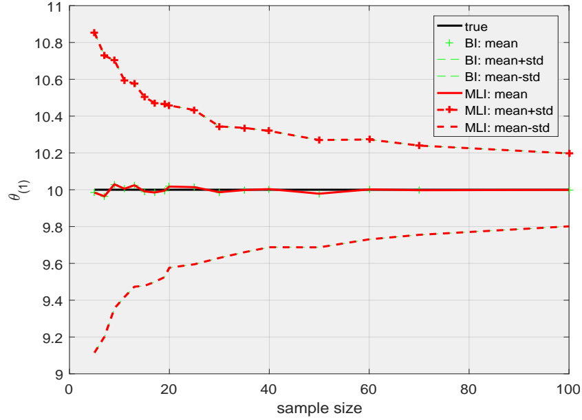
Figure 1. Estimation of the \theta(1) parameter of a normal distribution as a function of sample size. Both BI and MLI lead to the same estimator.
