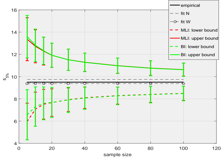
Figure 14. Application case. bounding the true s_{5\%} (complet sample: empirical quantile, weibull fit and normal fit) from sub-samples of the complete sample. Errors bars length of two times the standard deviation.
