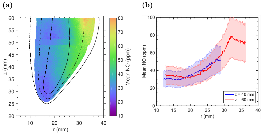
Figure 9: Conditionally averaged NO: (a) \chi_{NO} with conditional mean OH contours and centerline, (b) \chi_{NO} profiles with uncertainty bands.
