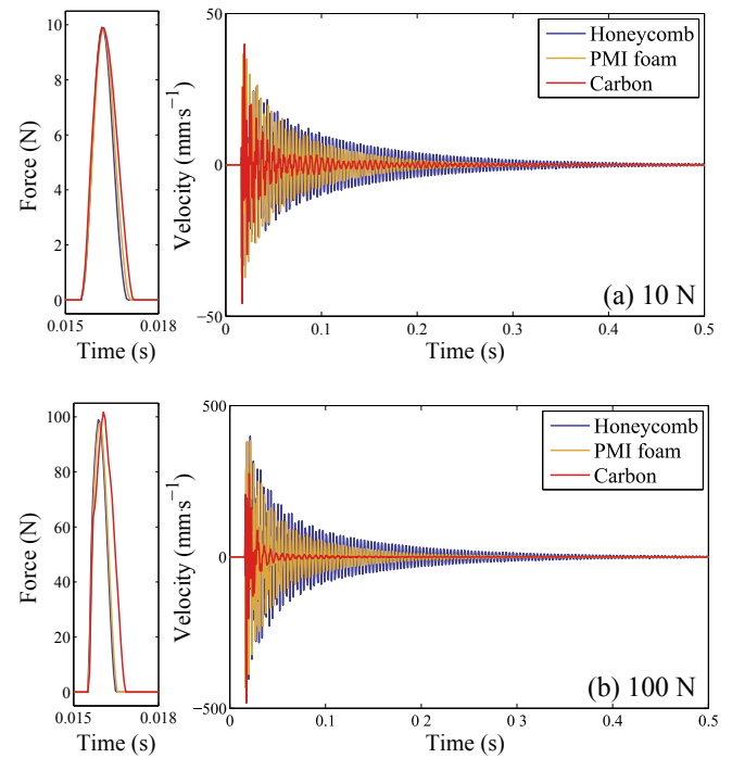
Figure 7: Transient response of sandwich beams with three different core materials to two impacts: (a) 10 N, 1.7 ms and (b) 100 N, 1.4 ms.
