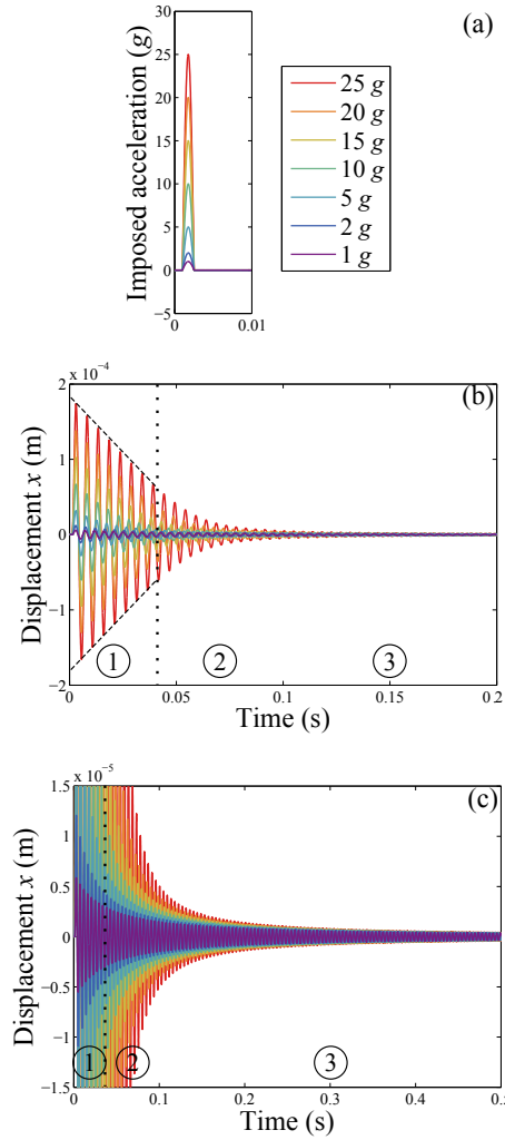
Figure 5: Simulated transient response of the single-degree-of-freedom system of Fig. 4: (a) imposed acceleration, (b) response for all amplitudes during 0.2 s and (c) zoom on the low response amplitudes during 0.5 s. Numbers indicate decay regimes: linear decay (1), and fast (2) and slow (3) "exponential" decay.
