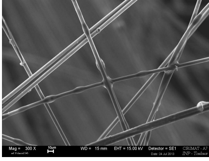
Figure 1: Scanning electron microscopy of the entangled cross-linked fibers after polymerization.
