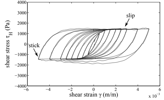
Figure 3: Shear stress-strain hysteresis loops obtained by removing the linear part of the shear stress: \tau_H = \tau - G_1\gamma with G_1 identified in Eq. (3). Loops measured at 20 Hz (grey line) and identified (black dotted line).
