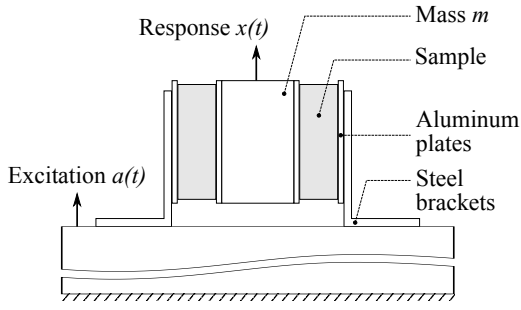
Figure 4: Principle of the studied single-degree-of-freedom system, including the entangled fiber samples in grey.
