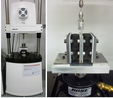
Figure 2: Experimental set-up for material characterization in shear.
