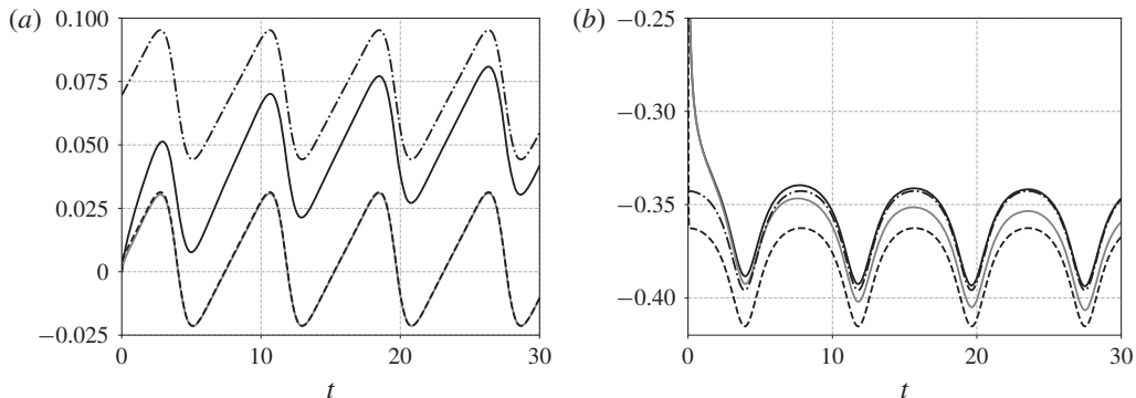
FIGURE 5. Evolution of (a) the e_1 -component, and (b) the e_3 -component of the slip velocity, \mathbf{u}_s , of a prolate spheroid with aspect ratio \lambda = 2 , as predicted using different approximations (time is normalized with the inverse of the shear rate, s^{-1} , and all velocities are normalized with the Stokes settling velocity of a sphere with radius a ). Black line: present unsteady theory; dash-dotted line: present quasi-steady theory; dashed line: prediction based on the Stokes quasi-steady drag; grey line: prediction based on the sum of the Stokes quasi-steady drag and the Basset–Boussinesq force.
