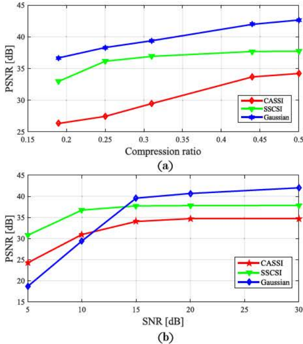
Fig. 9. PSNRs obtained with the proposed fusion method using CASSI, SSSCI and Gaussian sensing matrices for (a) different compression ratios (b) different SNR values.
