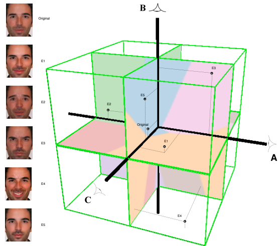
Fig. 1. Illustration of our 3-d representation space of emotion. Each color represents a discrete emotion ('happy', etc.). E_i are some generated facial expressions (left) mapped in our 3-d space (right). Better viewed in color.
