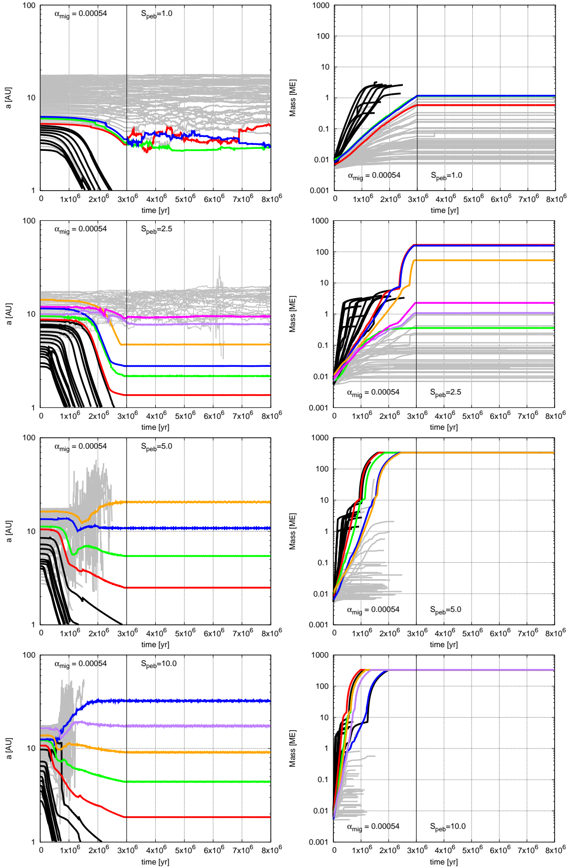
Fig. 4. Evolution of planetary systems with different pebble fluxes ( S_{\text{peb}} = 1.0, 2.5, 5.0 and 10.0 , top to bottom panels ) and \alpha_{\text{mig}} = 0.00054 in time. Semi-major axis ( left panels ) and planetary mass ( right panels ) of 60 planetary embryos as function of time. The gas disc lifetime is 3 Myr after injection of the planetary embryos. The black, grey and coloured lines show the same behaviour as bodies in Fig. 3.
