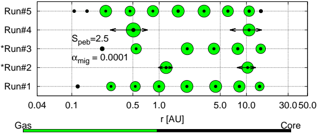
Fig. 10. Final configurations after 100 Myr of integration of all our simulations with \alpha_{\text{mig}} = 0.0001 and S_{\text{peg}} = 2.5 . The size of the circle is proportional to the total planetary mass (green) by the third root and to the mass of the planetary core (black) also by the third root. The runs marked with * are the example runs shown in Figs. 8 and 9, while the black arrows indicate the aphelion and perihelion positions of the planet calculated through r_p \pm e \times r_p . The here presented systems are a long-term integration of the same systems shown after 8 Myr ( S_{\text{peg}} = 2.5 ) of Fig. 7.
