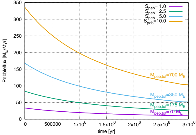
Fig. 1. Pebble flux as a function of time in our disc model with a gas disc lifetime of 3 Myr. We also show the upscaled pebble fluxes using the factor S_{\text{peb}} = 1.0 - 10.0 . Additionally, the total amount of pebbles M_{\text{peb,tot}} drifting through the gas disc during its lifetime of 3 Myr is marked.
