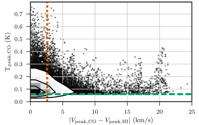
Figure 2. Distribution of the peak CO(2–1) brightness (with S/N > 3 ) versus the absolute difference in the HI and CO(2–1) peak velocities. The shaded region and contours indicate the regions containing the 1\sigma , 2\sigma , and 3\sigma limits of the distribution of points. Individual points show outliers beyond 3\sigma . The dashed horizontal line is the 3\sigma rms noise cutoff in the CO(2–1) data imposed to avoid spurious outliers in the velocity difference. The dotted vertical line is the CO channel width of 2.6 \text{ km s}^{-1} . The CO velocities are preferentially located at or near the HI velocities. However, there remain a number of high S/N outliers with a large velocity difference. These outliers occur when the CO emission is associated with a different HI component than the brightest HI peak.
