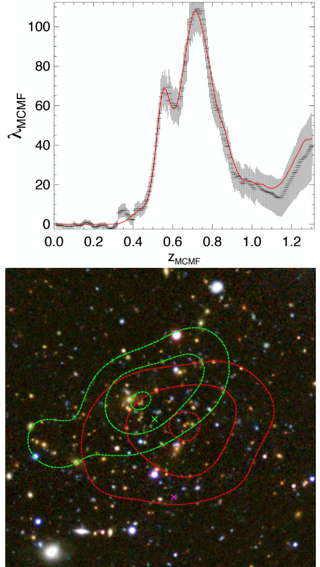
Figure 18. Top panel: Lambda versus z as produced by MCMF for MARD J020216.7–540216 (SPT-CL J0202–5401). The red line represents the best model fit for two clusters at z = 0.54 and z = 0.70 . Bottom: DES grz pseudo-colour image of the central 3x3 arcmin region, centred on the SPT position (green cross). The 2RXS position is marked with a magenta cross. Green contours show the galaxy density for RS galaxies at z = 0.54 and red contours are used for z = 0.7 .
