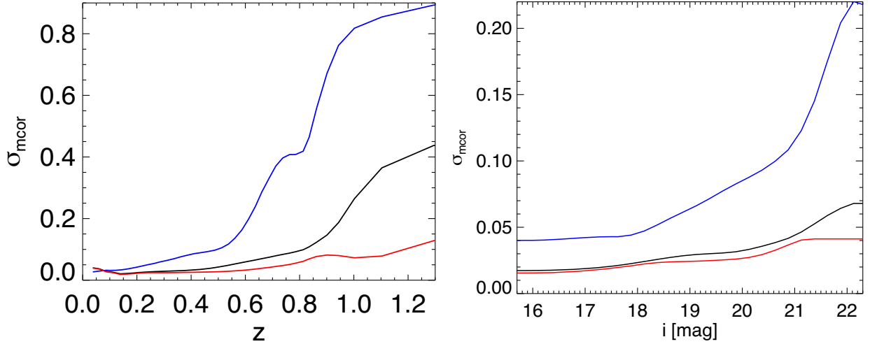
Figure 2. Left: Measurement error corrected colour width of RS galaxies at m^* for g-r (blue), r-i (black) and i-z (red). Right: Measurement error corrected colour width versus magnitude at z = 0.31 . The characteristic magnitude m^* is i \approx 19 mag.
