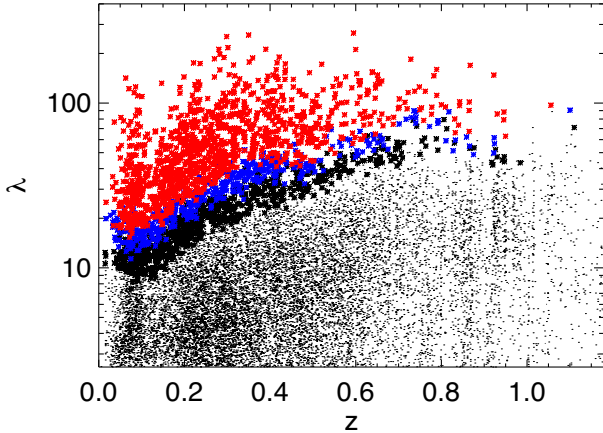
Figure 8. Richness versus redshift of the MARD-Y3 cluster catalogue for selections f_{\text{cont}} < 0.2 (black), f_{\text{cont}} < 0.1 (blue), and f_{\text{cont}} < 0.05 (red). Multiple detections of clusters are excluded, no X-ray, AGN, or star exclusion is applied.
