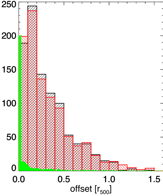
Figure A9. Offset distribution of RM matched systems between default MCMF and 2RXS (black), RM and 2RXS (red), and default MCMF and RM (filled, green). The green histogram was scaled down by a factor of 2.3 to fit into the plot.
