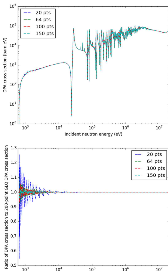
Figure 3. Neutron elastic scattering DPA cross sections of ^{56}\text{Fe} performed with 20, 64, 100, and 150 points Gauss-Legendre quadrature (upper) and the corresponding ratios to the 200-point Gauss-Legendre quadrature calculation (lower).
