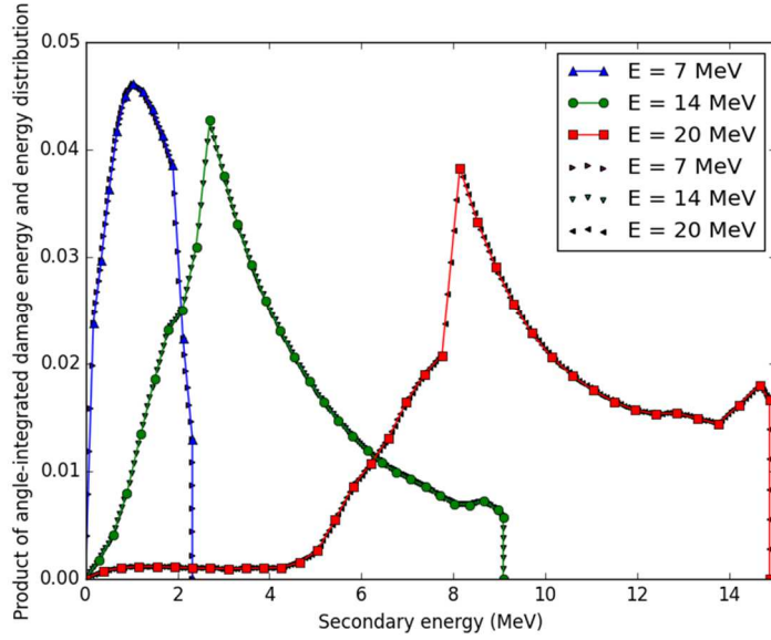
Figure 7. Energy distribution of the angle-integrated damage energy, i.e. \int_{-1}^1 f(E, E_1, \mu) E_a(E, E_1, \mu) d\mu , for 7 MeV, 14 MeV, and 20 MeV neutron continuum inelastic scattering of ^{56}\text{Fe} . The larger points are calculated based on the energy grid in JEFF-3.1.1. The smaller points are computed at 5 evenly inserted energies.
