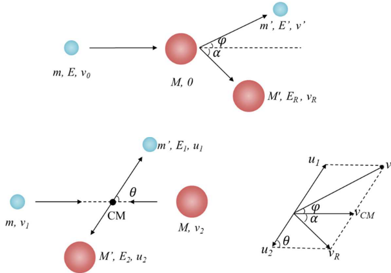
Figure 1. Schemes of the collision in the Laboratory (upper) and Center of Mass (lower) frames
