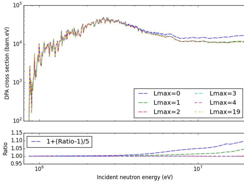
Figure 16. First level neutron inelastic scattering DPA cross sections of ^{56}\text{Fe} performed with different maximum Legendre ( L_{\text{max}} ) polynomials.
