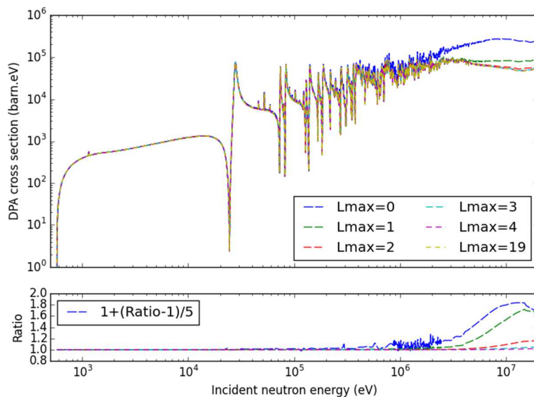
Figure 14. Neutron elastic scattering DPA cross sections of ^{56}\text{Fe} performed with different maximum Legendre ( L_{\text{max}} ) polynomials.
