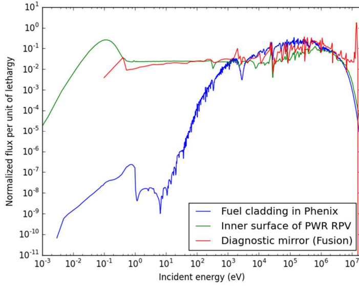
Figure 20. Neutron spectra in the fuel cladding of Phenix reactor, in the inner surface of RPV in a typical PWR, and in the diagnostic mirror of a fusion reactor.
