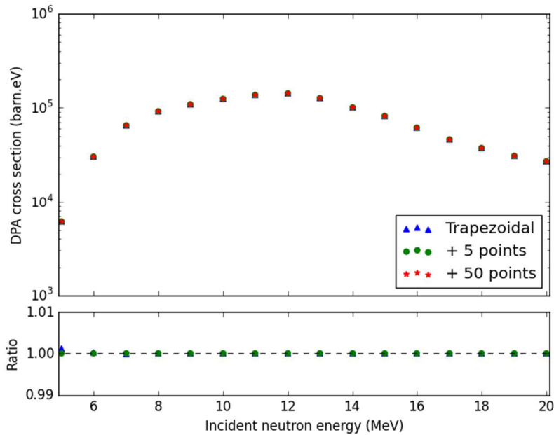
Figure 8. Neutron continuum inelastic scattering DPA cross sections of ^{56}\text{Fe} computed with the trapezoidal integration by using the energy grid in ENDF, 5 and 50 evenly inserted points in each interval. The corresponding ratios are calculated over the DPA with 50 inserted points.
