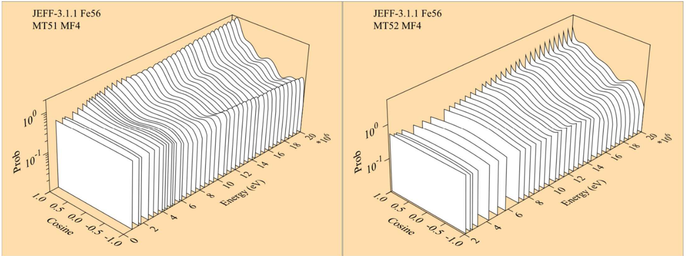
Figure 15. Angular distributions of the neutron first (left) and second (right) levels inelastic scattering reactions (MT51 and MT52) of ^{56}\text{Fe} in JEFF-3.1.1 [7]
