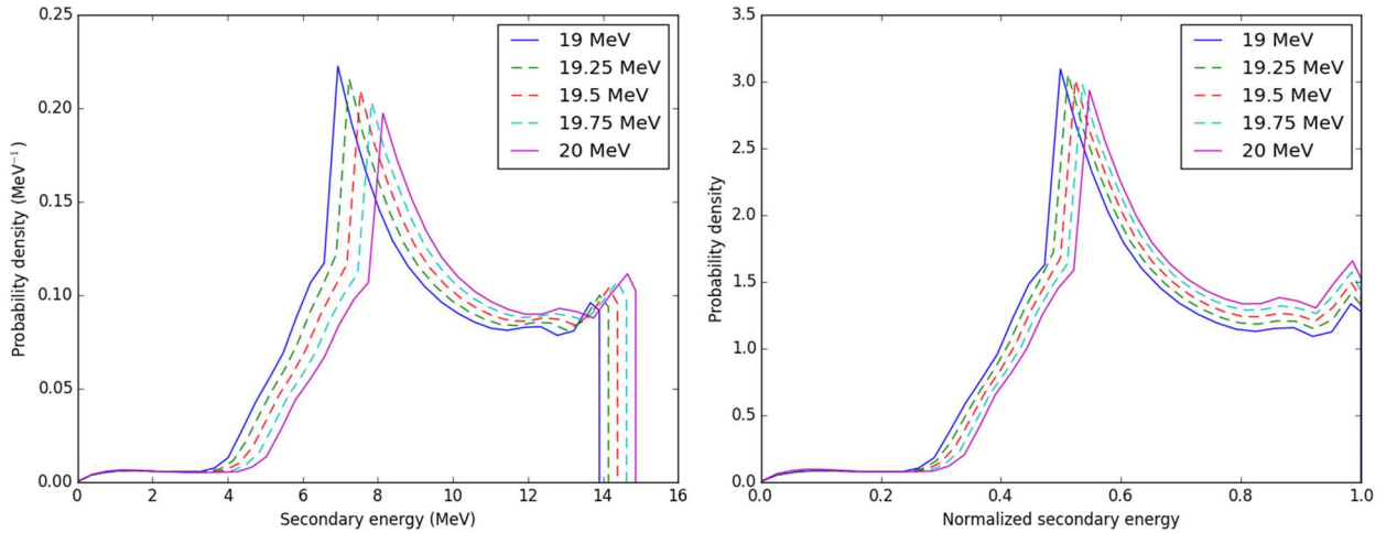
Figure 11. Same results as Figure 10 but with PUBI
