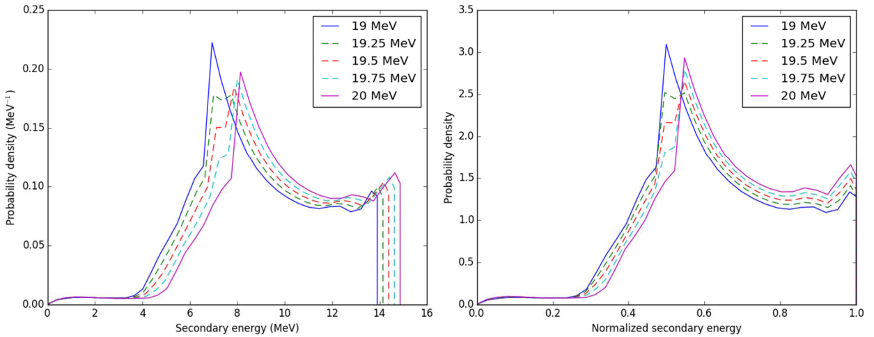
Figure 10. UBI of angle-integrated energy distributions of incident energy between 19 and 20 MeV neutron continuum inelastic scattering with ^{56}\text{Fe} . The right figure uses the normalized secondary energy to intuitively show the peak values.
