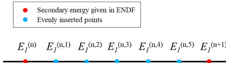
Figure 6. Scheme of 5 evenly inserted points between two neighbor secondary energies given in ENDF
