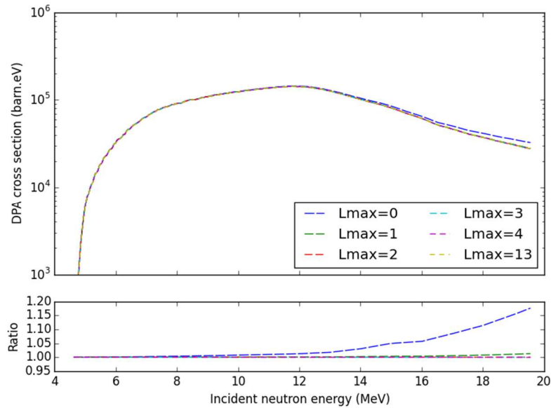
Figure 17. Neutron continuum inelastic scattering DPA cross sections of ^{56}\text{Fe} performed with different maximum Legendre (Lmax) polynomials and the corresponding ratios to the DPA with full order Legendre polynomials.
