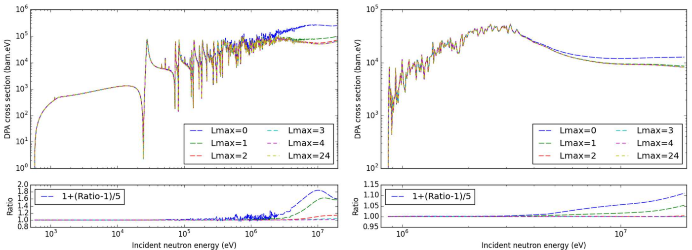
Figure 18. Neutron elastic scattering (left) and first-level inelastic scattering (right)-induced DPA cross sections of ^{56}\text{Fe} with different Lmax using ENDF/B-VIII
