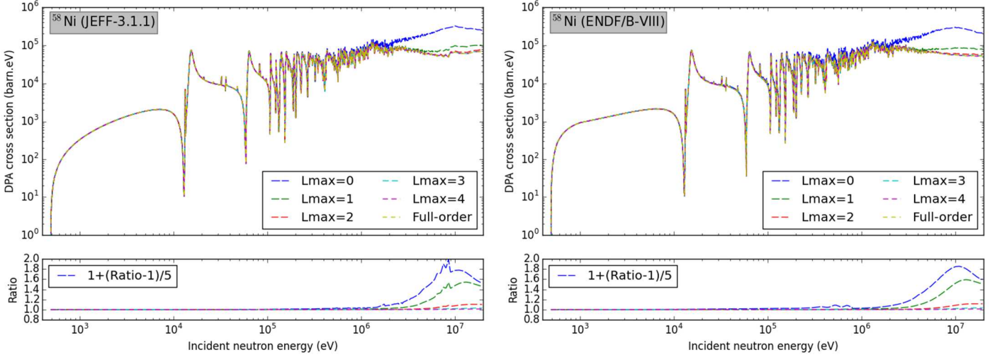
Figure 19. Neutron elastic scattering-induced DPA cross sections of ^{58}\text{Ni} with different Lmax using JEFF-3.1.1 (left) and ENDF/B-VIII (right)
