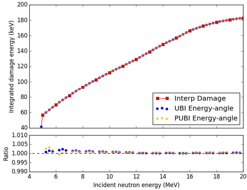
Figure 12. Energy-angle-integrated damage energy. The red square points are computed with energy-angular distributions given in the ENDF, the red line is linear interpolation between two incident energies, the blue circles (orange stars) are calculated with UBI (PUBI) energy-angular distributions. The lower figure plots the ratio of blues circles to the interpolated damage energies.
