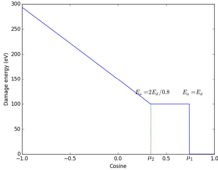
Figure 2. Damage energy of ^{56}\text{Fe} versus the cosine in CM for 5 keV neutron elastic scattering
