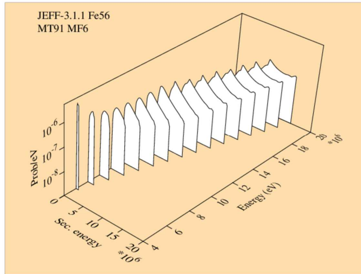
Figure 5. Energy distribution of the continuum inelastic scattering of ^{56}\text{Fe} in JEFF-3.1.1 plotted by NJOY-2016
