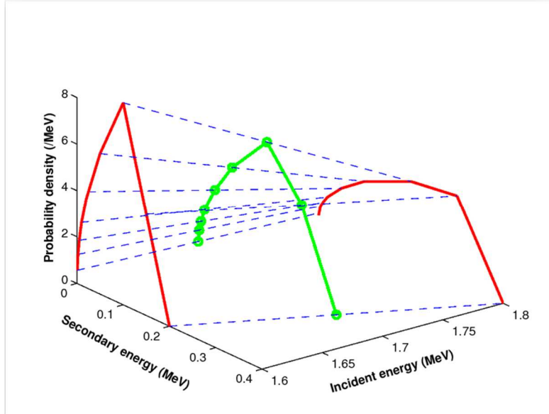
Figure 9. Scheme of the interpolation of energy angular distributions. Red lines represent the data given in ENDF, the green points are interpolated data.
