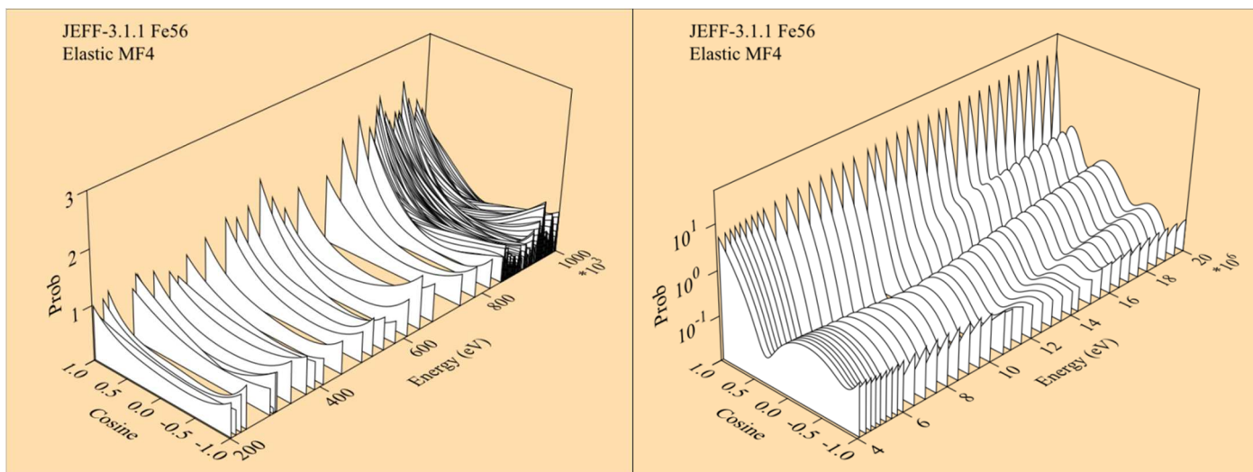
Figure 13. Angular distributions of the neutron elastic scattering reaction of ^{56}\text{Fe} in JEFF-3.1.1 [7] with the incident energies in the interval [200 keV, 1 MeV] (left) and [4 MeV, 20 MeV] (right) plotted by NJOY-2016 [26].
