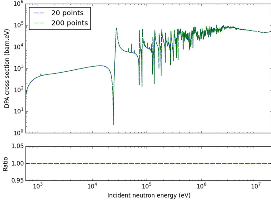
Figure 4. Neutron elastic scattering DPA cross sections of ^{56}\text{Fe} performed with 20 and 200 points Gauss-Legendre Quadrature based Piecewise Integration (GLQPI).
