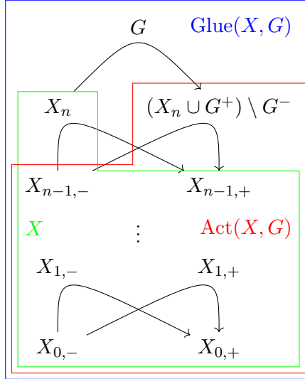
Figure 3: Cells involved and their movements in Theorem 2.1.1
