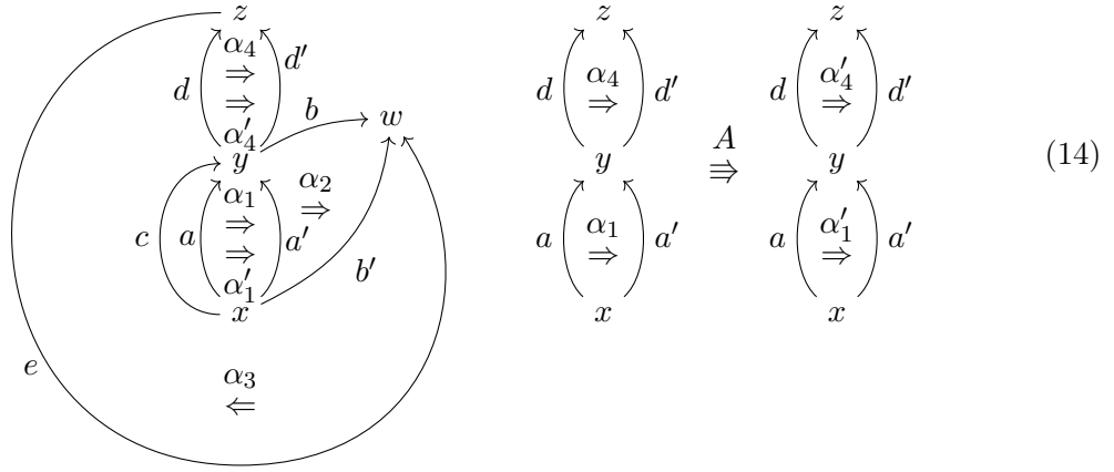
Figure 2: A problematic \omega -hypergraph
