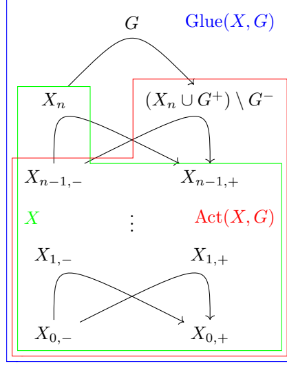
Figure 1: Cells involved and their movements in Theorem 2.2.3
