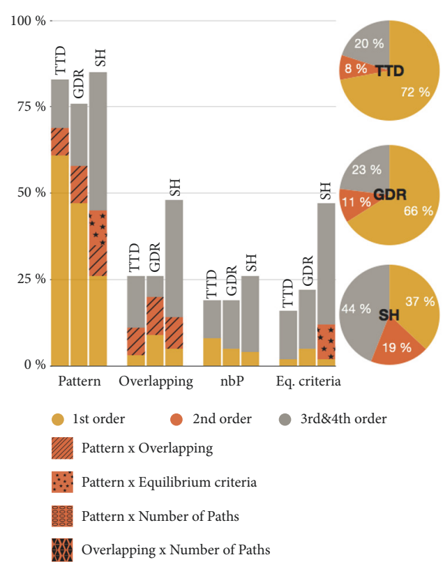
FIGURE 16: Presentation of Sobol indices for three representative case studies.
