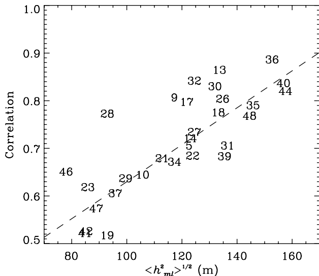
Figure 6. Scatterplots between the correlation of surface vorticity from the model and the estimate of surface vorticity derived from SST and (top) the RMS of vorticity, (middle) the RMS of wind stress, and (bottom) the RMS of the mixed layer depth. Dashed lines correspond to a linear fit between observations. In the first plot, boxes with values of vorticity RMS above 0.15 have not been used to compute the linear fit; in the middle plot, boxes 9, 13, 17, and 19 have not been used; in the bottom plot, box 28 has not been used. Numbers correspond to the box identification number.
