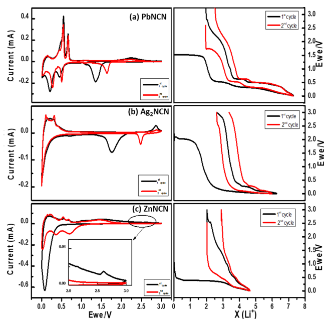
Figure 3. Cyclic voltammetry ( 0.05\text{ mV s}^{-1} ) and the corresponding galvanostatic profile ( C/10 , corresponding to 1 mol of Li reacted per mole of compound in 10 h) of (a) \text{PbNCN} , (b) \text{Ag}_2\text{NCN} , and (c) \text{ZnNCN} .
