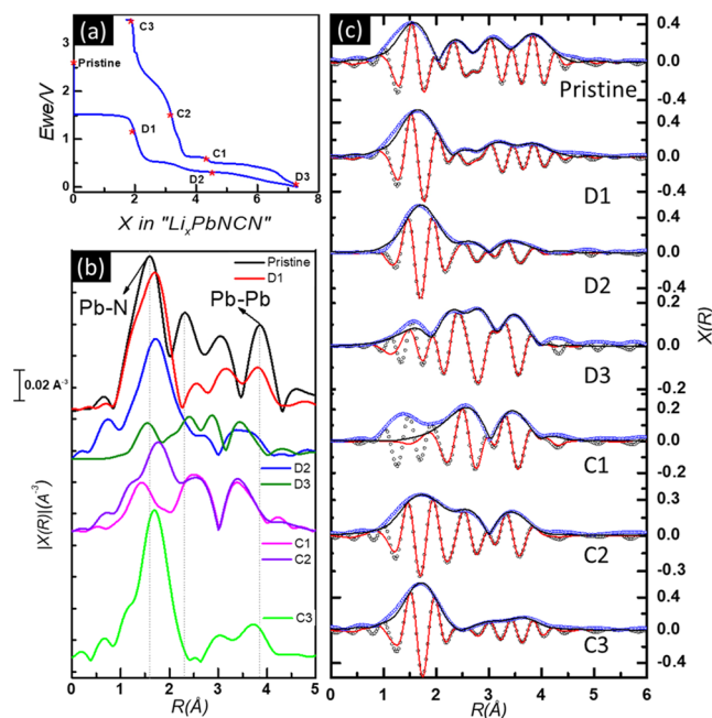
Figure 6. Galvanostatic profile (a), |\chi(R)| plots (b) and fits of the EXAFS R -space portion of the ex-situ data of PbNCN in (c). Blue and black circles are experimental real and imaginary parts, respectively. Black and red lines are fitted real and imaginary parts respectively.
