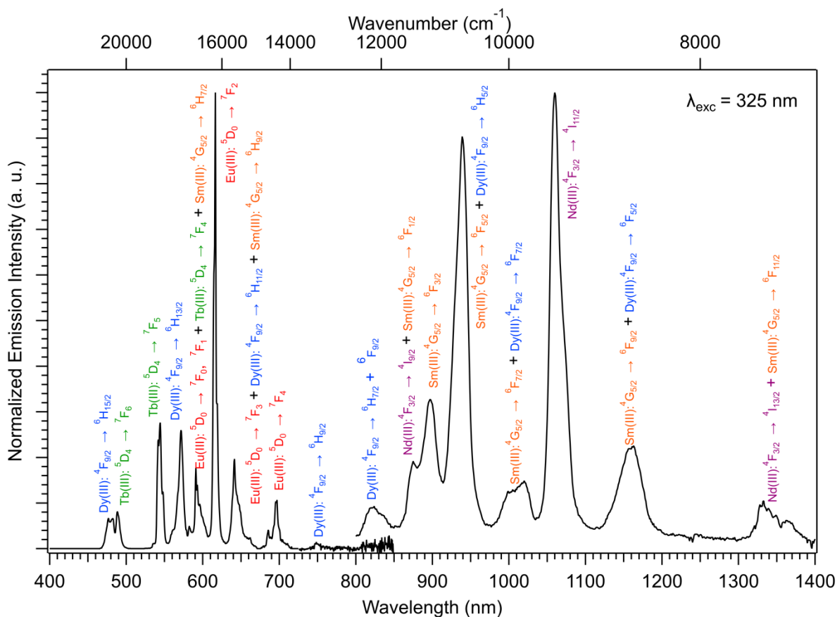
Figure 9. Emission spectrum, recorded at room temperature under UV irradiation ( \lambda_{\text{exc}} = 325 \text{ nm} ), in the visible and IR regions, of [\text{Nd}_{0.4}\text{Sm}_{0.4}\text{Eu}_{0.3}\text{Gd}_{0.2}\text{Tb}_{0.1}\text{Dy}_{0.6}(\text{mip})_3]_{\infty} . \tau_{\text{obs}}(\text{Tb}) = 0.08(1) \text{ ms} and \tau_{\text{obs}}(\text{Eu}) = 0.12(1) \text{ ms} . Spectra normalized on the most intense peak of the visible (450-850) and NIR regions (850-1600 nm), respectively.
