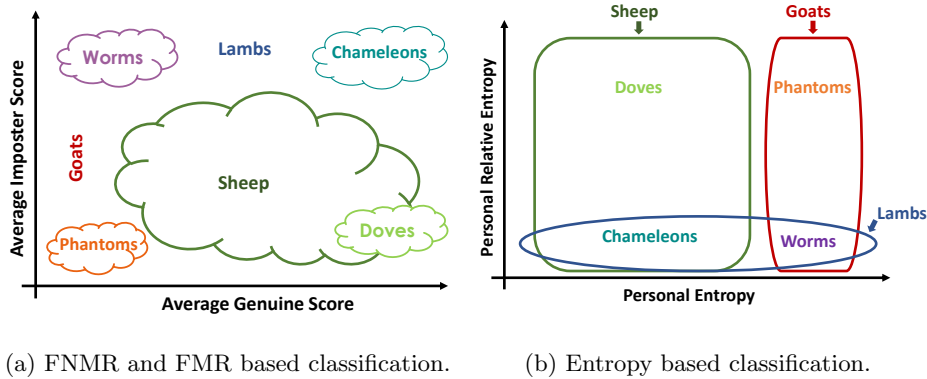
Figure 2: Large animal groups distinguished by Doddington zoo according to [30].
