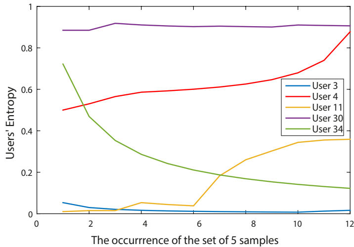
Figure 3: Personal entropy of some users of WEBGREYC database.
