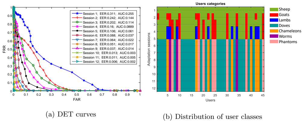
Figure 8: Achieved performances when considering scenario 2 for WEBGREYC database.
