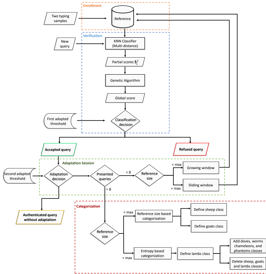
Figure 4: Description of the keystroke authentication process
