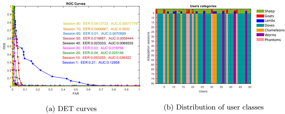
Figure 6: Achieved performances and the distribution of users classes for CMU database.
