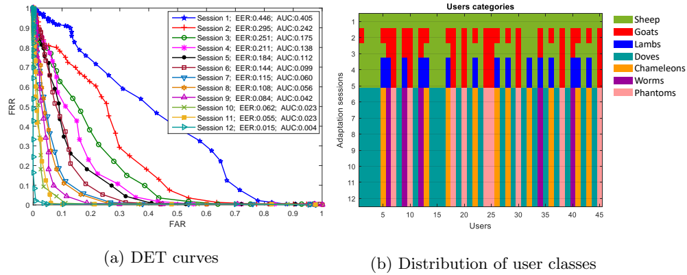
Figure 7: Achieved performances when considering scenario 3 for WEBGREYC database.
