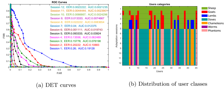
Figure 5: Obtained performances and the distribution of users classes for WEBGREYC database.
