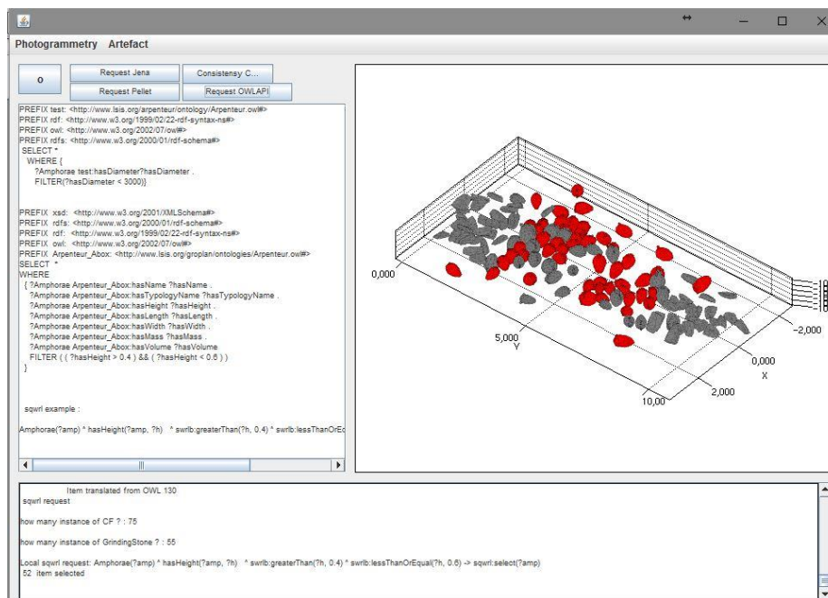
Fig. 1. 3D visualization of a spatial request in SWRL:
