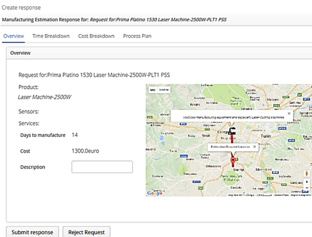
Figure 17. Estimation Overview
