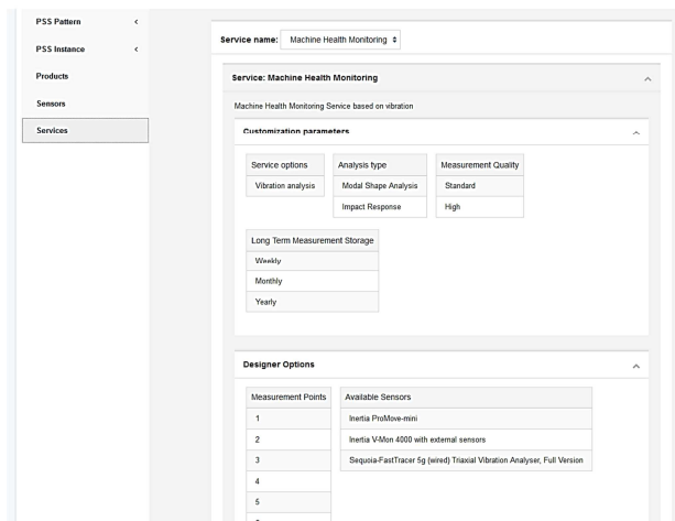
Figure 12. Service description as a PSS requirement
