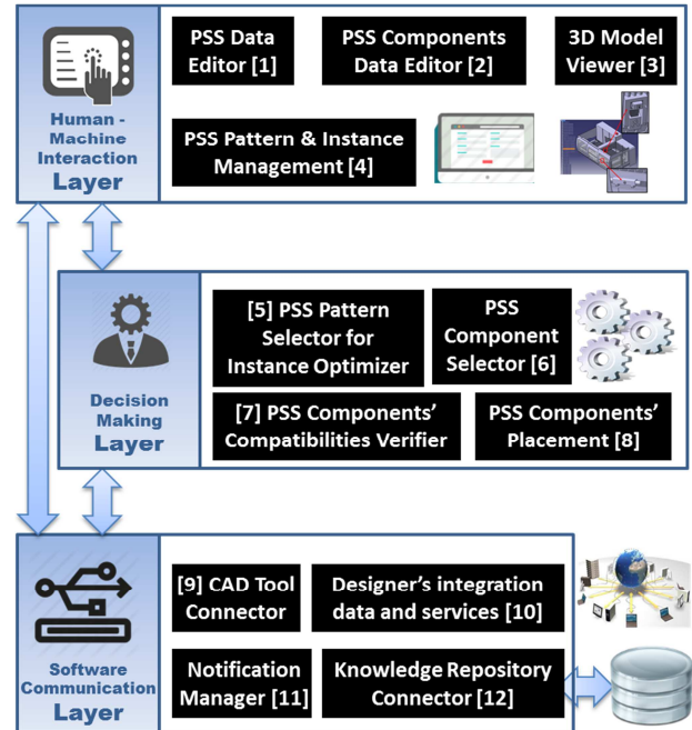
Figure 5. Global architecture of the Designer component
