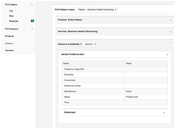
Figure 13. Partial view of PSS pattern solution
